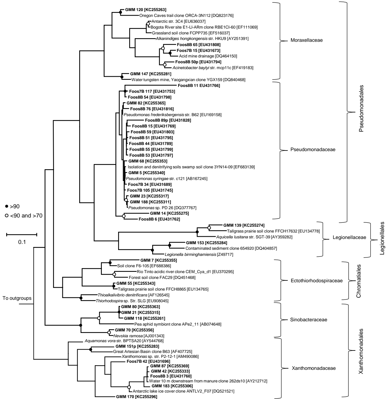
Supplemental Figure 2. Phylogenetic reconstruction among 16S rRNA gene sequence retrieved from moonmilk from Grotta della Foos and Bus della Genziana (labeled in bold) compared to closest relatives affiliated to the Gammaproteobacteria . Accession numbers for relatives are included. The scale bar corresponds to distance.
