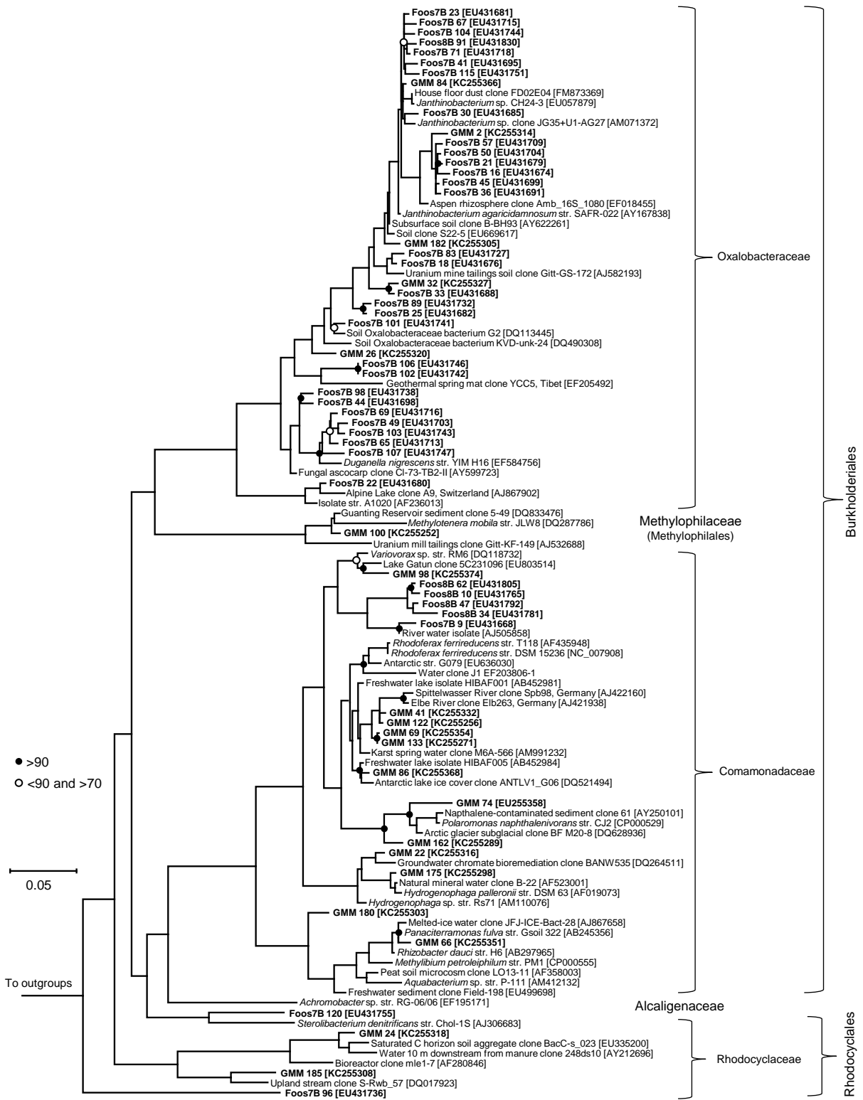
Supplemental Figure 1. Phylogenetic reconstruction among 16S rRNA gene sequence retrieved from moonmilk from Grotta della Foes and Bus della Genziana (labeled in bold) compared to closest relatives affiliated to the Betaproteobacteria . Accession numbers for relatives are included. The scale bar corresponds to distance.
