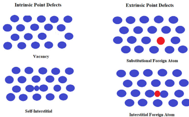
Figure 3 Point defects.
