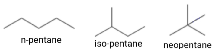
Figure 8: Pentane Conformers
