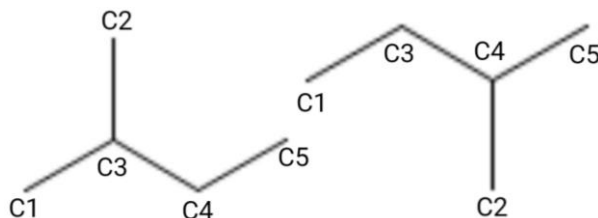
Figure 3: C2 Conformers
