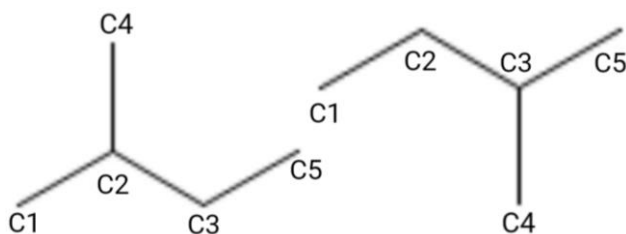
Figure 5: C4 Conformers
