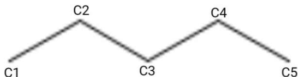
Figure 1: Basic Structure of Pentane
