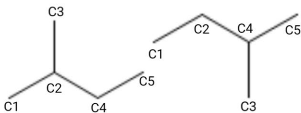
Figure 4: C3 Conformers
