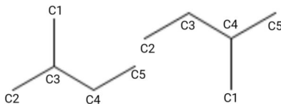
Figure 2: C1 Conformers
