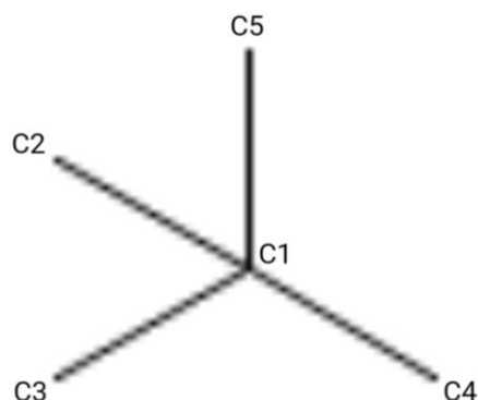
Figure 7: Tetrahedral Conformer (C1)
