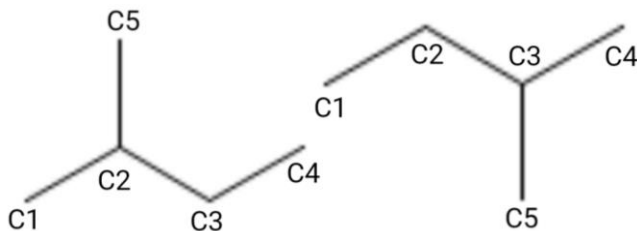
Figure 6: C5 Conformers
