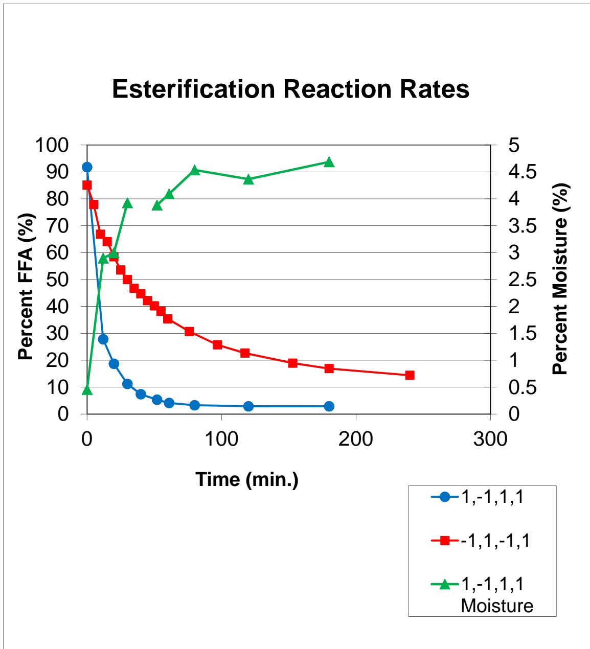
Figure 21: Esterification reaction rate for two factor combinations
