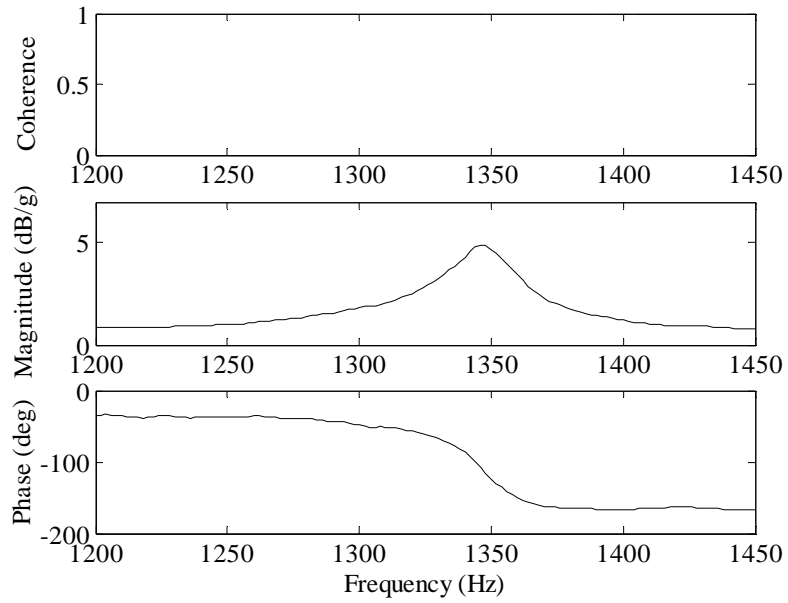
Figure 117. Frequency response plot of solar cell specimen 24 over the narrowband range of 1200-1450 Hz; experimental run number 35.
