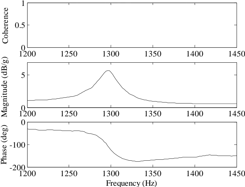
Figure 101. Frequency response plot of solar cell specimen 19 over the narrowband range of 1200-1450 Hz; experimental run number 19.
