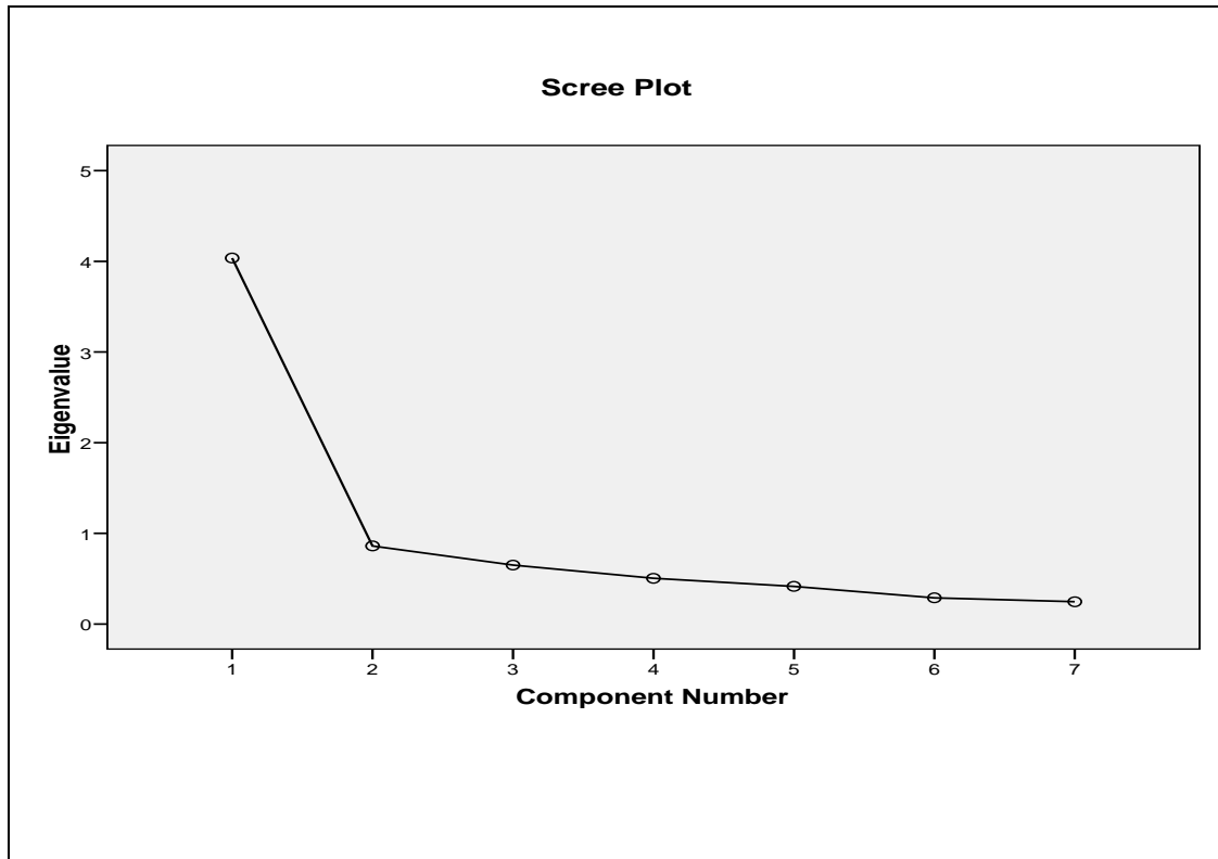
Figure 1: Scree Plot
