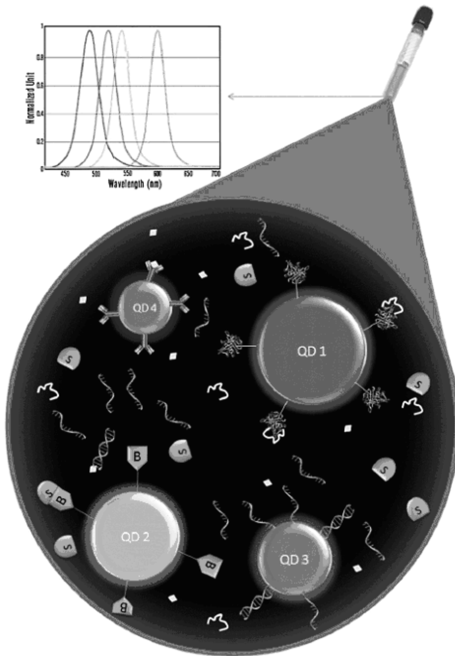
Figure 2.19. Schematic diagram for simultaneous detection of different targets in a serum sample using QDs of different sizes, functionalized with different recognition moieties: peptide/ protein (QD1), biotin (QD2), oligonucleotide (QD3), or antibodies (QD4). Abbreviations: B (biotin), S (streptavidin). Emission spectra of different sized-QDs (1–4) are shown in the upper left corner [85].
