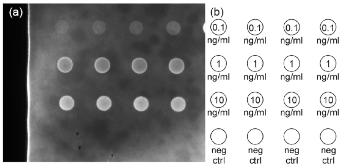
Figure 2.13 Example of fluorescent microscope image (mag. 2.5x) of the small part of an array printed from micro array printer (QD655 + IL10 complex) with 100 \mu m spot diameter (a), spots description (b) [64]
