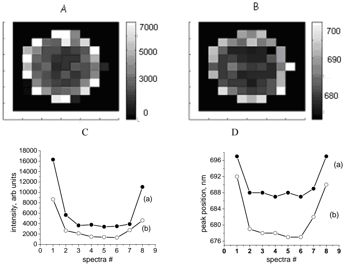
Figure 3.23. Photoluminescence (PL) maps of a conjugated to CAV1 antibodies sample stored for 3 days at 50 0 C: A – PL intensity; B – PL peak position. The linescans of (a) 30 minuets dried and (b) stored for three days at 50C conjugated sample: C – PL intensity; D – PL peak position.
