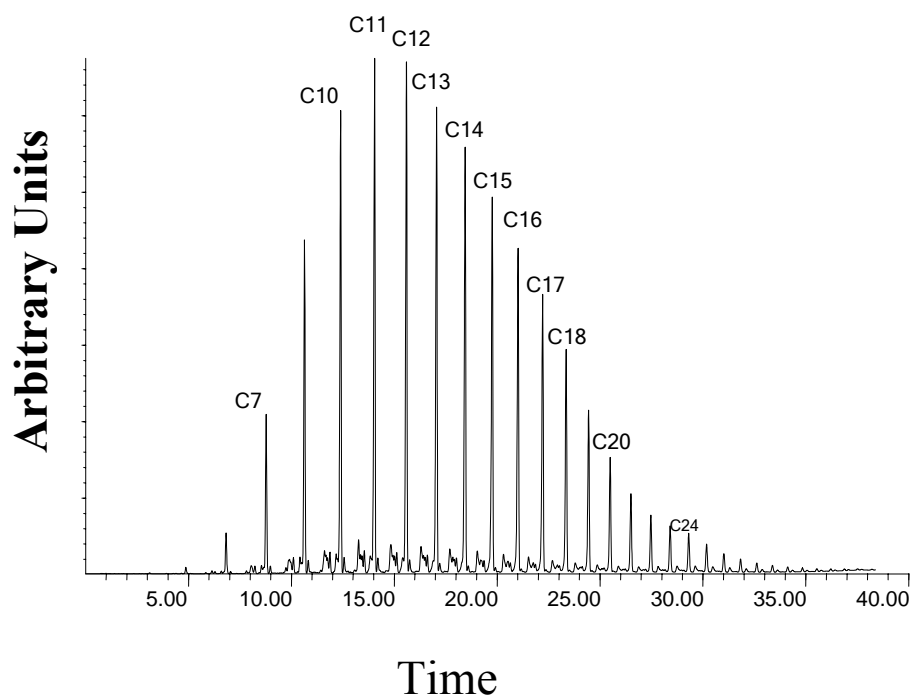
Figure 18. GC analysis of liquid product obtained from FTS of Sample 4
