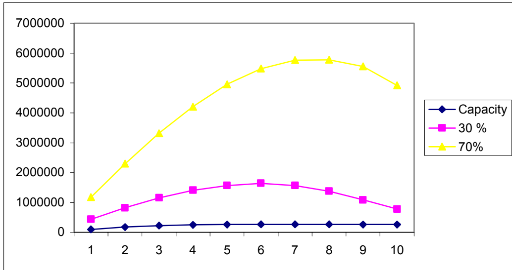
Figure 10: Benefit for 6 Lanes Toll Plaza with Multiple Additional ETC Lanes
