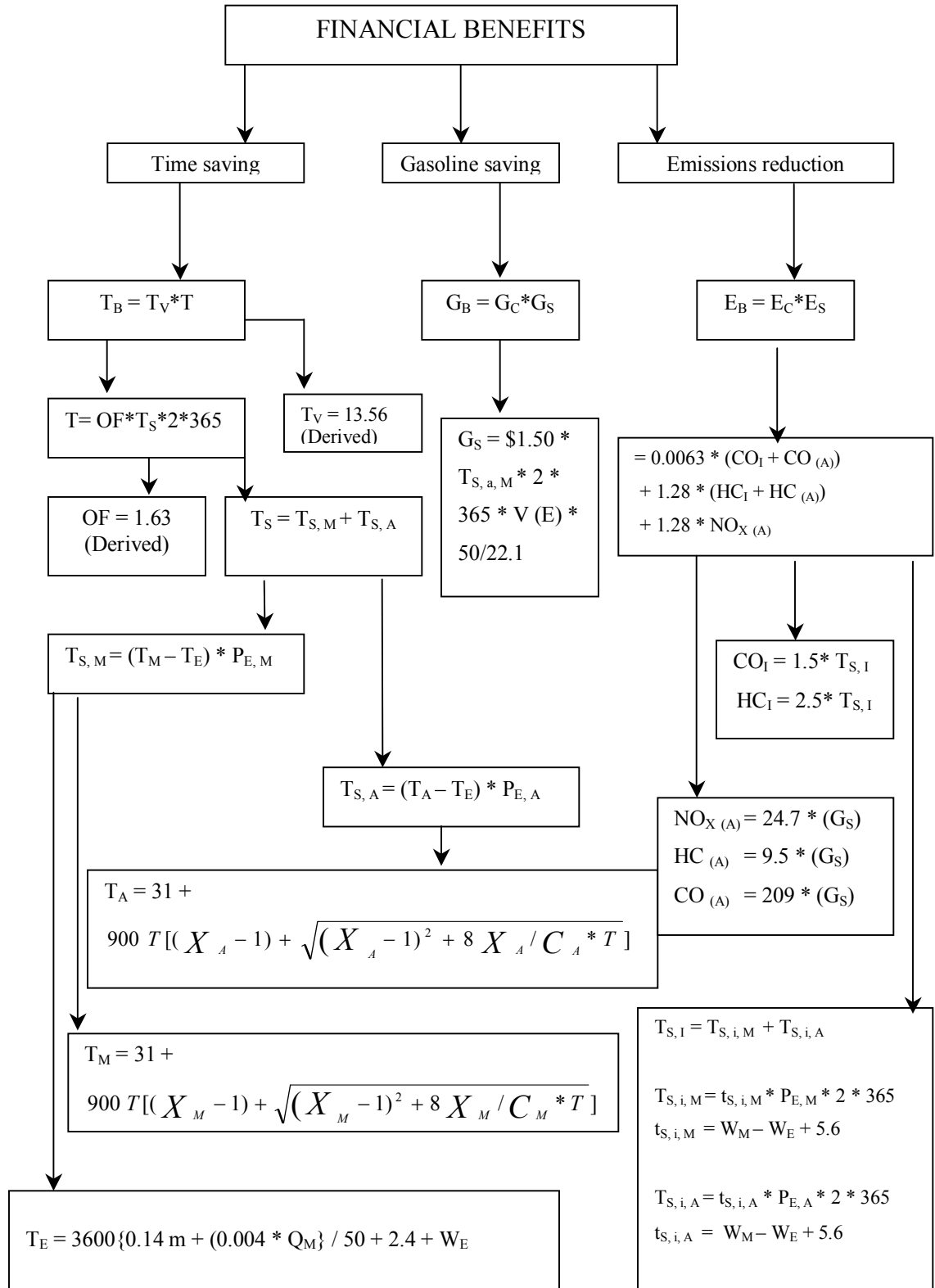
Figure 6: Model Components
