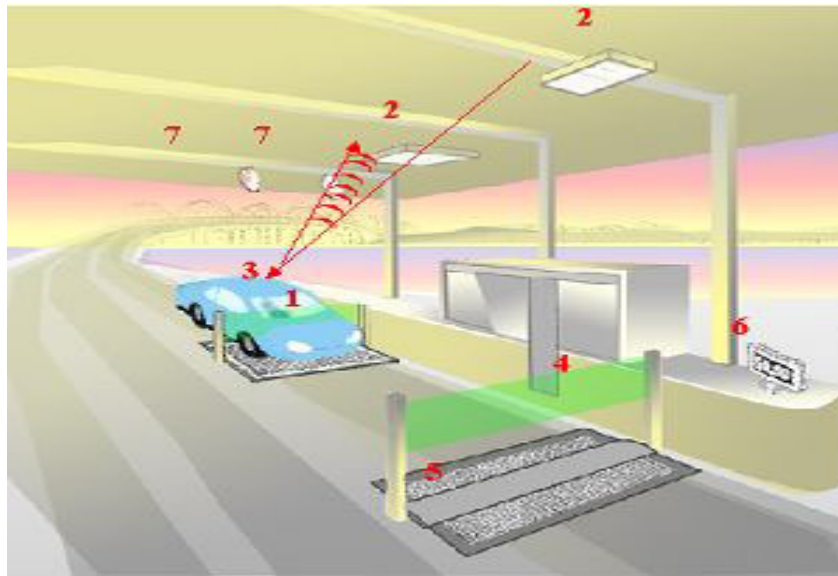
Figure 3: ETC System Operation
