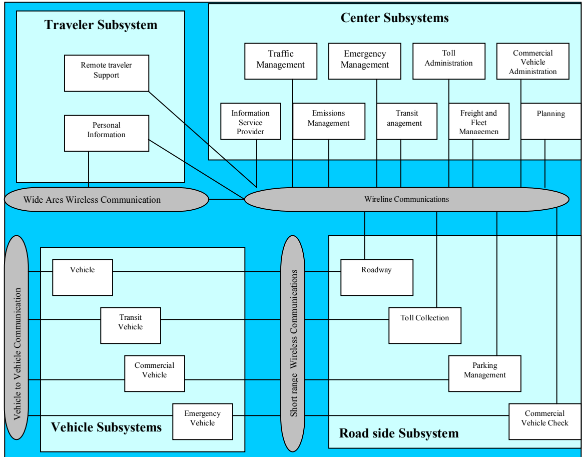
Figure 2: Transportation and Communication Layers of Physical Architecture
