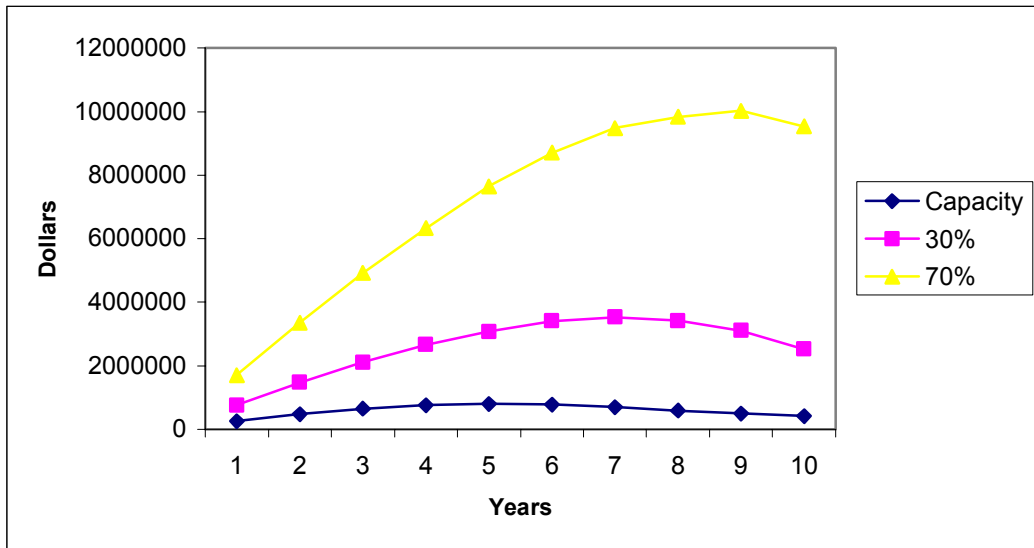
Figure 11: Benefit for 7 Lanes Toll Plaza with Multiple Additional ETC Lanes
