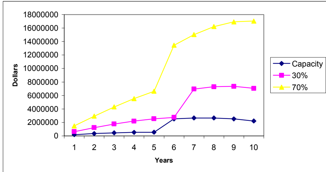
Figure 8: Benefit for 5 Lanes Toll Plaza with Multiple Converted ETC Lane
