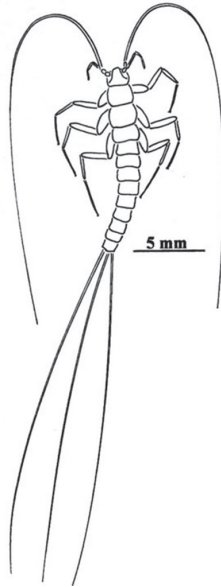
Figure 2. Anelpistina quinterensis is one of the most troglomorphic described species of nicoletiids. This relatively large eyeless insect is albino and has extremely elongated appendages. Its habitat is restricted to very humid portions of the caves such as mud banks. It is doubtful that it can survive in an epigeal environment. Its habitat probably reflects connectivity within a karstic area throughout geologic times and during the evolutionary history of the species.
