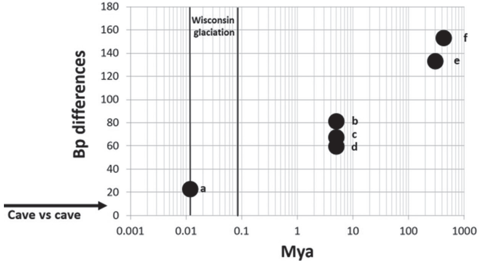
Figure 3. Base pair differences versus estimates of divergence in nicoletioids. Base pair differences in the 16S rRNA fragment is plotted against estimates of divergence times millions of years ago (Mya). Molecular clock calibrating points were extracted from: a populations of Anelpistina musticensis that got separated into different islands when the sea level rose after glacial times 12,000 years ago (Espinasa et al. 2011) b and c species of Prosthecina and d species of Anelpistina from Baja California that got separated from the mainland species when the Gulf of Cortes formed 5 mya (Espinasa et al. 2009) e time when nicoletioids arose from a common ancestor with Lepismatids 302 mya (Regier et al. 2010), and f time when insects arose from a common ancestor with anostraca in the Silurian-Ordovician boundary 427 mya (Gaunt and Miles 2002). The lower arrow indicates the 11–12 bp differences between the Sierra de Guatemala and the Sierra de El Abra Anelpistina populations. Such sequence difference is consistent with a common origin very recently, less than 12,000 years ago, and therefore after the environmental disturbances of the ice age.
