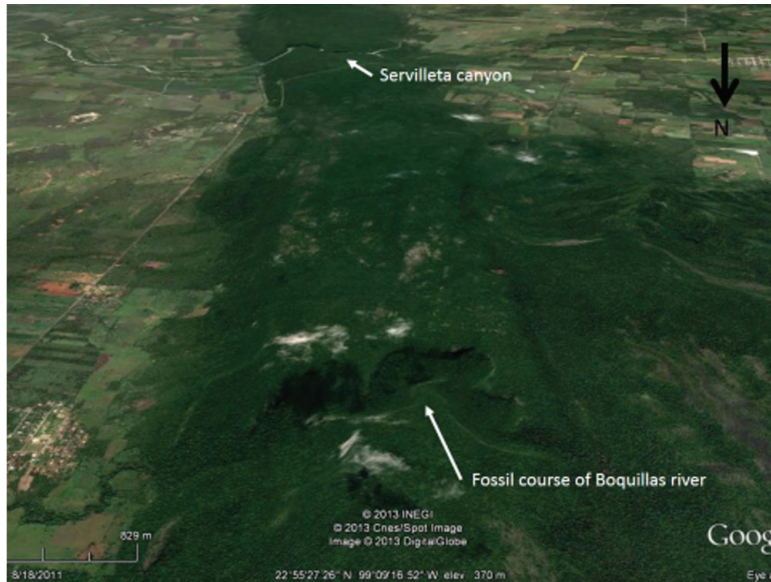
Figure 4. The Boquillas River has changed its course throughout time. The Boquillas River currently separates the karstic areas of Sierra de Guatemala from the Sierra de El Abra. In the upper part of the figure, the Boquillas River is seen crossing the sierras through the Servilleta canyon. On the bottom part of the figure, a fossil canyon indicates the river's ancient course. Caves that in the past connected the Sierra de El Abra in the south to the Sierra de Guatemala in the north were only recently geologically truncated by the erosion of the new river course. Limestone is restricted to the green forested hills.
