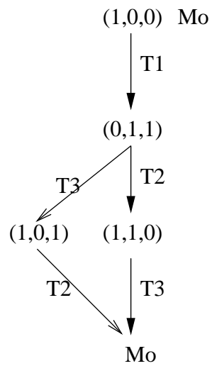
Figure A.2. Reachability Tree
