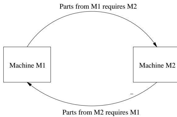
Figure 1.1. Deadlock
