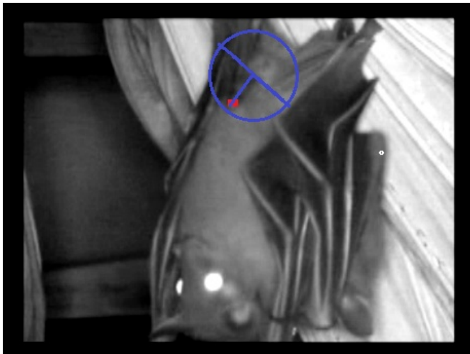
Figure 3: Snapshot photograph from video of C. sphinx mating. Geometric representation of the restricted range demonstrated by the articulated
