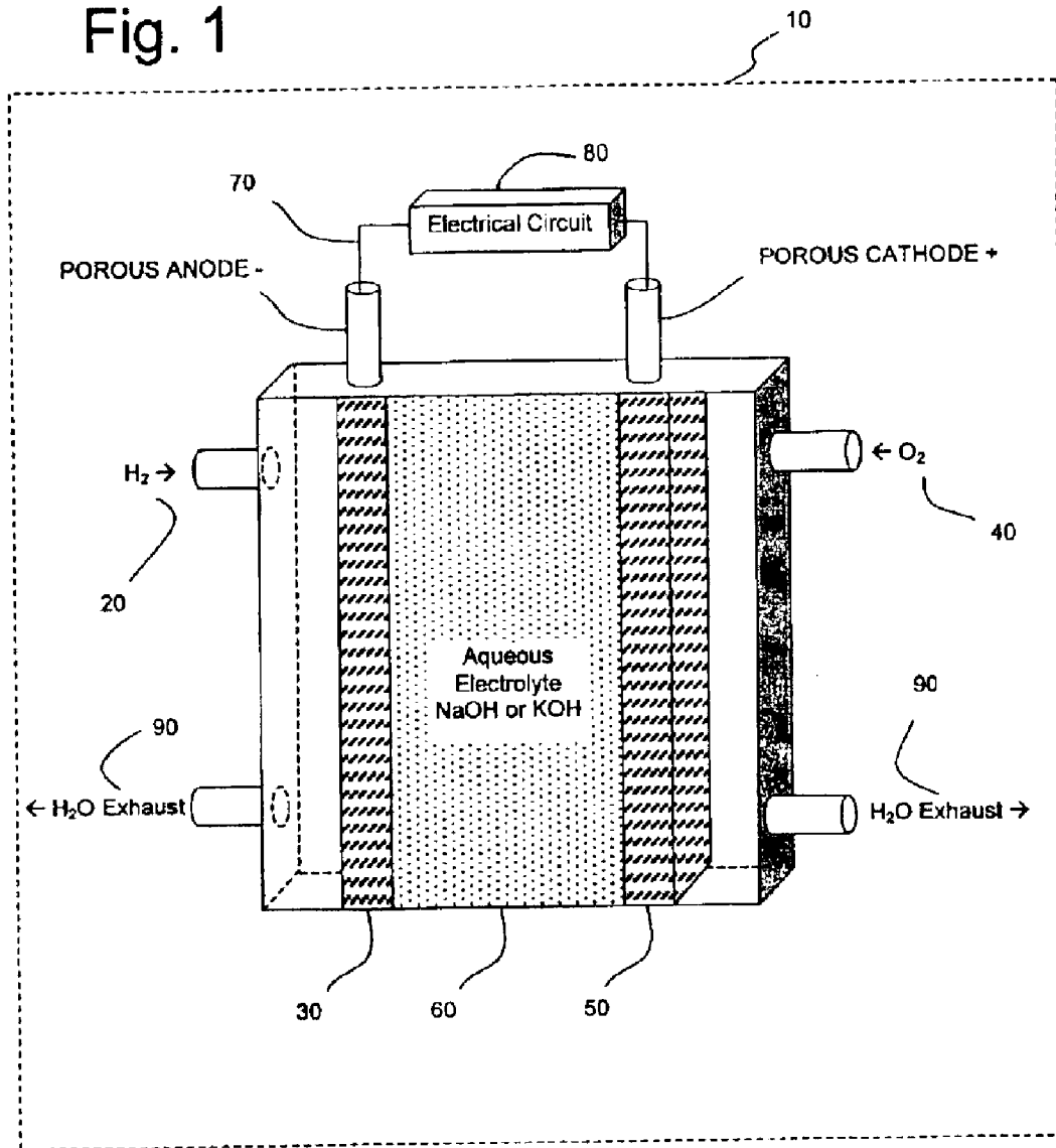
(Prior Art Hydrogen/Oxygen Fuel Cell)
