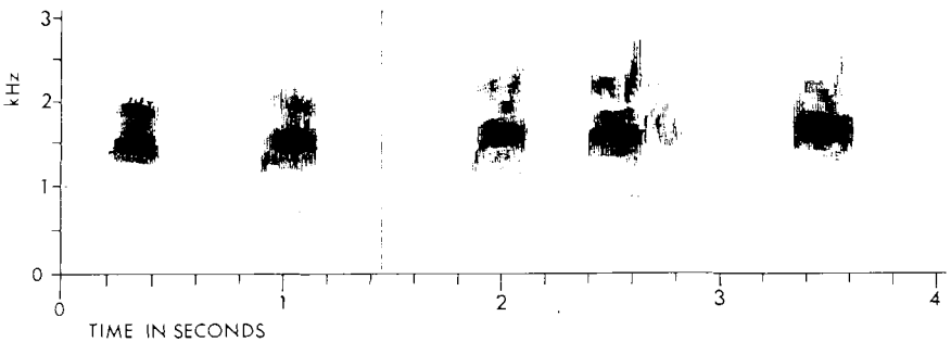
Figure 5. Sonograms of typical calls of: left, 6 month-old Tamaulipas Crows (in January 1988, molt completed); right, adult Tamaulipas Crows, illustrating that they were indistinguishable from each other.
