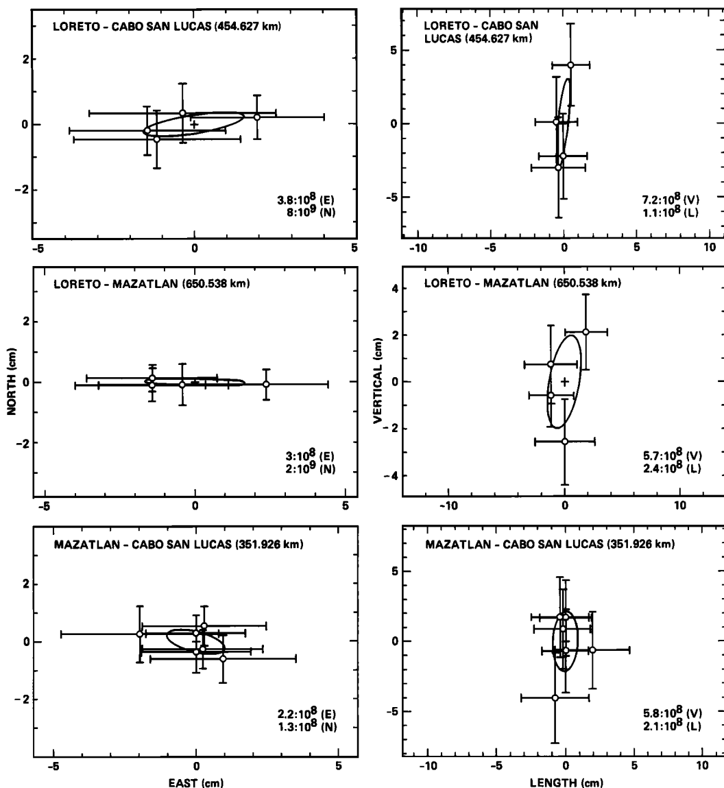
Figure 1. Baseline component (E, N, V) and length (L) solutions for each of the three Gulf baselines using combined carrier phase and pseudorange data. Solutions for each day are plotted about the weighted mean of all solutions. The errors are described in the text. Only four days of high-quality data are available for Loreto. The one standard deviation repeatabilities are in parts per 10^8 (or 10^9 ). Note that for the east-west Cabo San Lucas to Mazatlan baseline, the east component and length are essentially identical.
