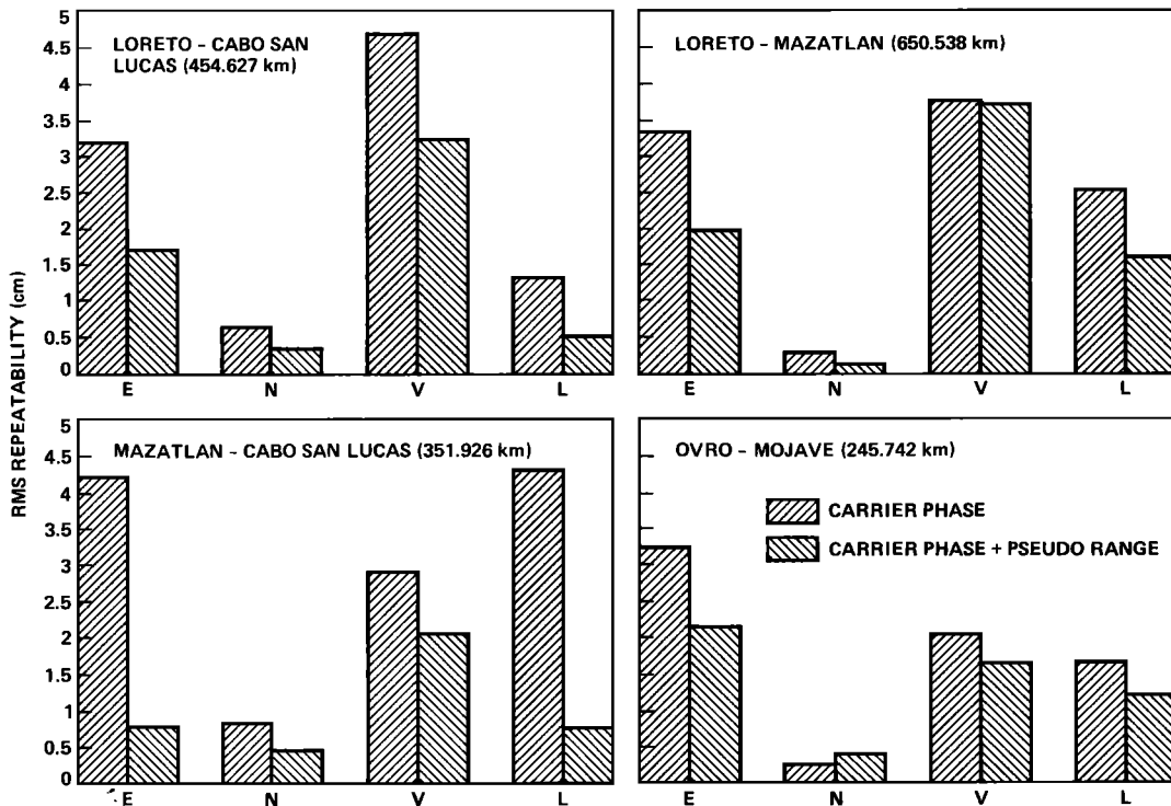
Figure 2. Histogram of baseline component (E, N, V) and length (L) repeatabilities using carrier phase data with and without pseudorange data.
