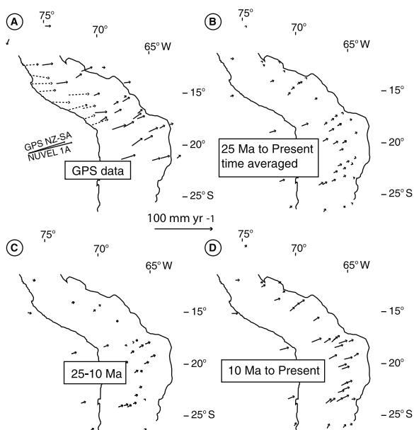
Figure 2. Comparison of geodetic and geologic velocities within the Central Andes. (a) shows the GPS velocities with respect to the stable interior of South America and the convergence vector for the Nazca plate with respect to South America derived from the GPS data and predicted by the NUVEL-1A global plate motion model. Dashed vectors are transiently elastically loaded and not directly comparable in magnitude to the geologic data (b) shows the average geologic velocities over the past 25 Ma. (c) and (d) show average velocities for a two step displacement field, 25–10 Ma and 10 Ma–Present.
