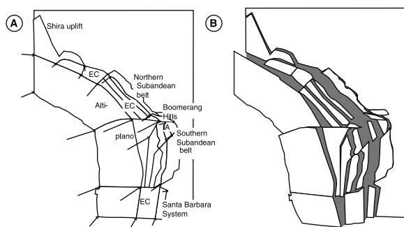
Figure 1. (a) Present day position and names of the blocks used in the Andean geological displacement model. EC - Eastern Cordillera, IA - Interandean Zone. Arrows show geologic, finite displacements at block edges. (b) Retro deformed state of the block model at 25 Ma. Grey zones are block boundary zones representing fold and fault displacements internal to each block.
