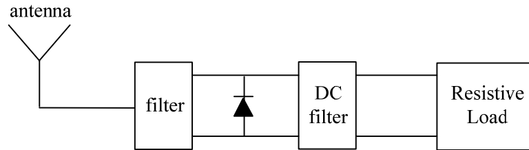
Figure 1.3: Rectenna Block Diagram, [13]
