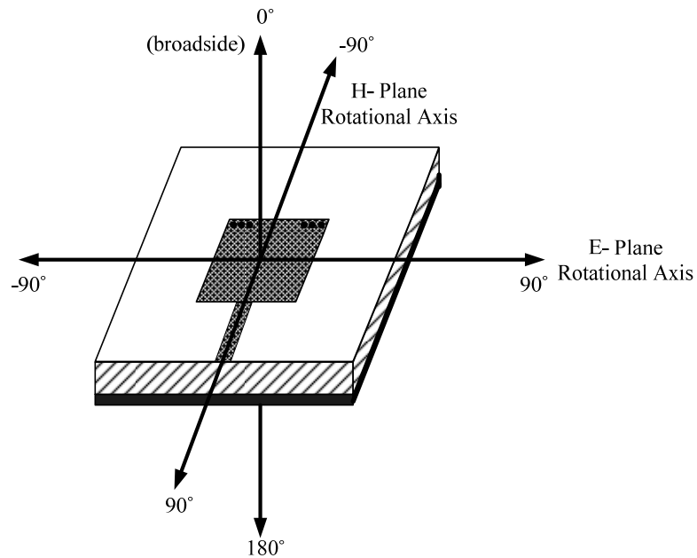
Figure 2.15: Axis Definition for Antenna Measurements
