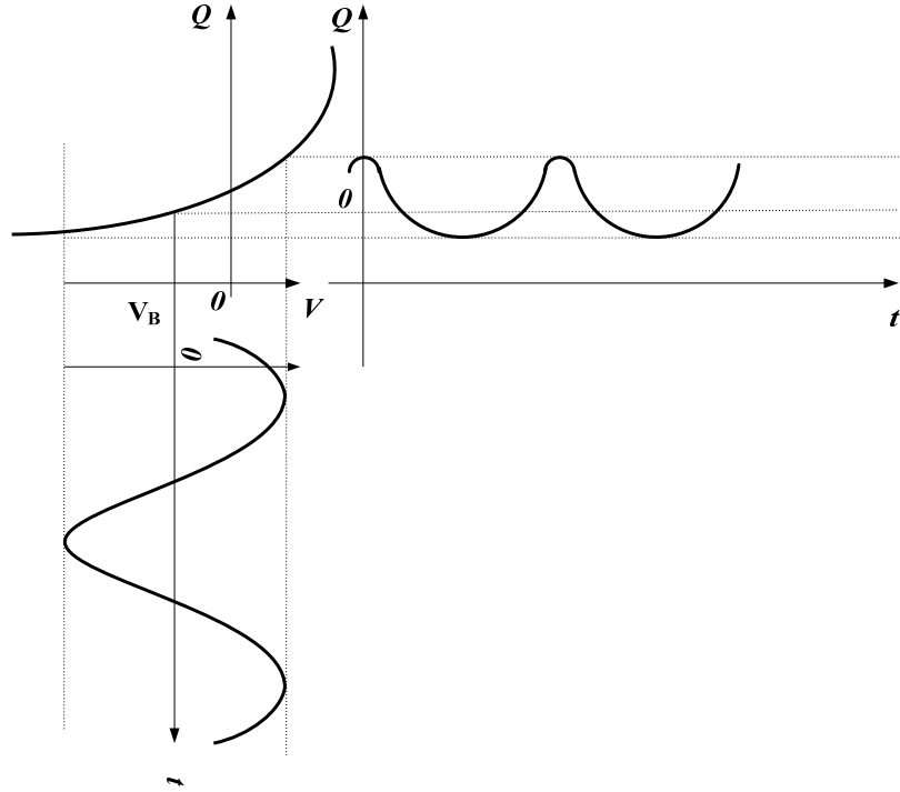
Figure 1.1: Operating Principle of a Frequency Multiplier Using Nonlinear Capacitance, [3]
