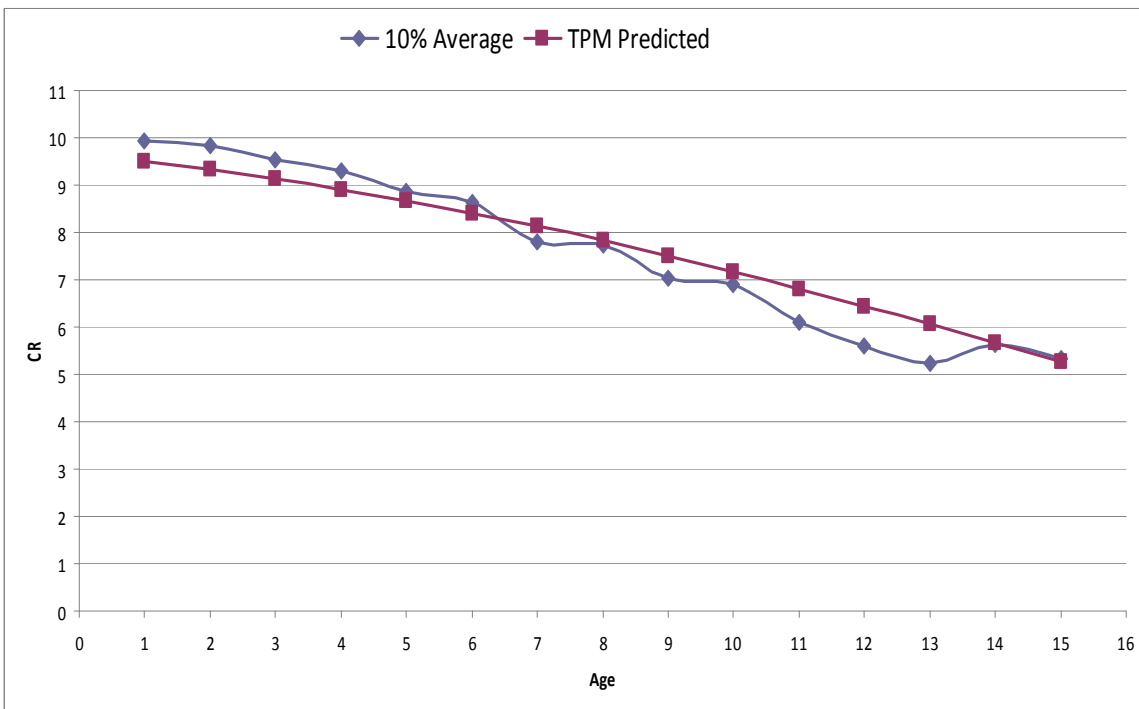
Figure 8-B. Comparison with the 10% verification set at their 3 rd duty cycle (structural integrity deficient sections)
