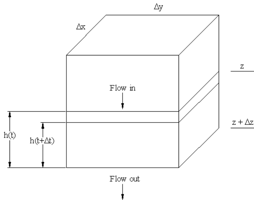
Figure 13 Diagram explaining variables of the mass balance method for calculating seepage into and out of a surficial aquifer.
