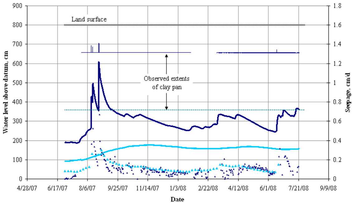
Figure 23 Well hydrographs for the post office site. The thin dark line represents the location of the top of the clay pan as well as the location of the shallow well sensor, the dotted line is the approximate bottom of the clay pan, the thick dark line is surficial well hydrograph, the thick light line is the Floridan well hydrograph, the dark dots are the seepage values calculated using mass balance method, and the light dots are the seepage values calculated using the head gradient method.
