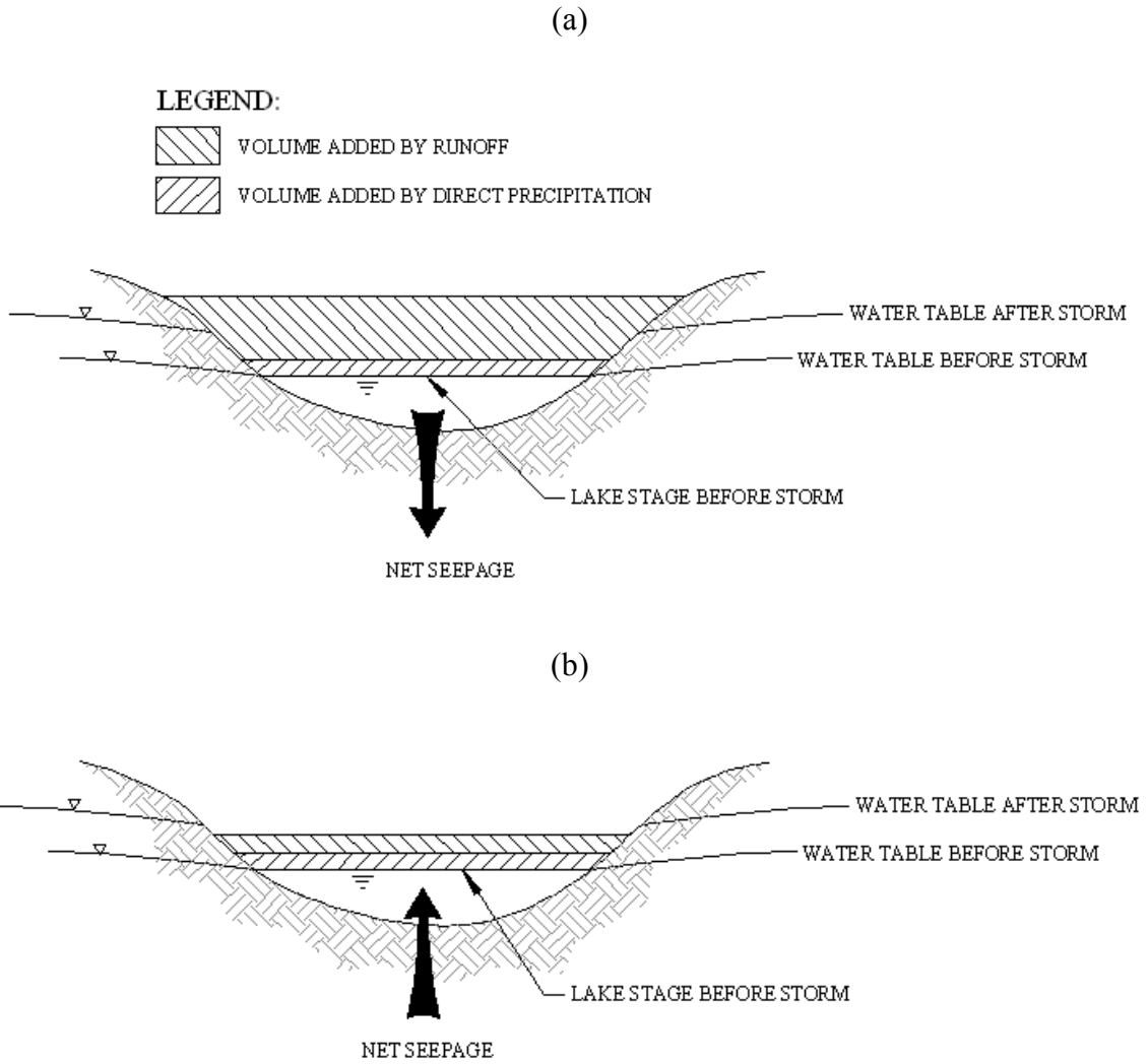
Figure 21 Diagram of the response of seepage to rain events in lakes receiving (a) large and (b) moderate amounts of runoff. Not to scale.
