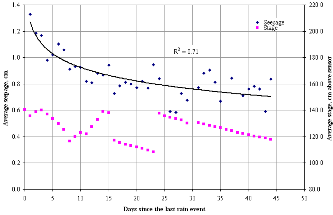
Figure 16 Botanical Gardens: correlation between time since precipitation and seepage and stage.
