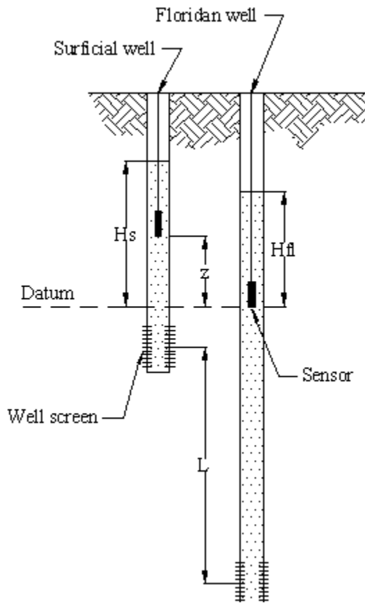
Figure 14 Two-wells diagram showing variables used in Darcy's Law.
