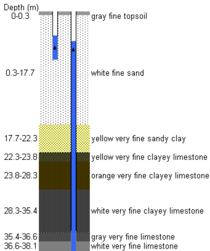
Figure 7 Soil layers and well depths (cross-section) at Site 4.
