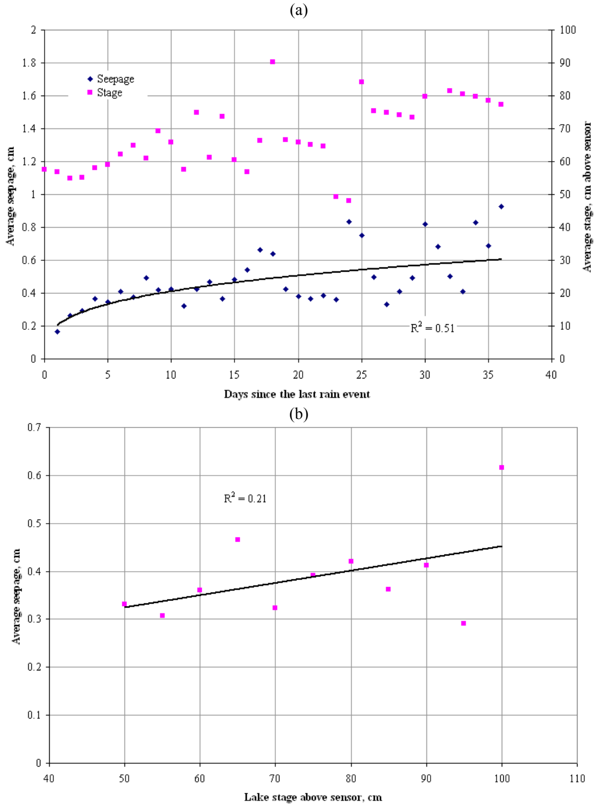
Figure 22 Lake Wimauma: correlation between (a) the time since the preceding precipitation event and seepage and stage, and (b) seepage and lake stage.
