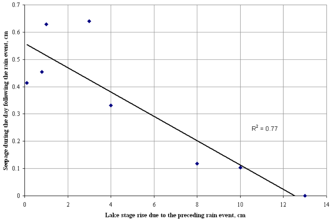
Figure 20 Lake Park: correlation between seepage during the day following the rain event and the magnitude of the event.
