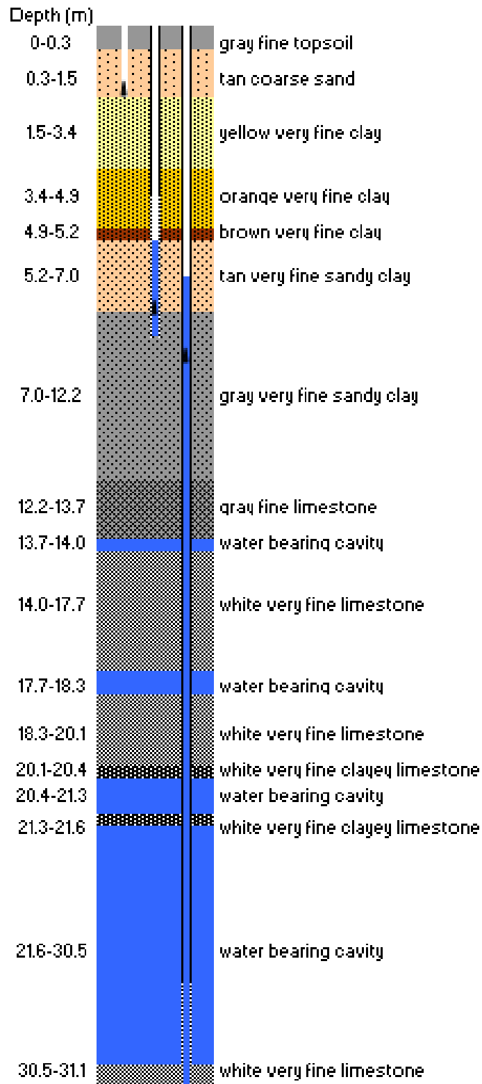
Figure 4 Soil layers and well depths (cross-section) at Site 3. Not to scale.
