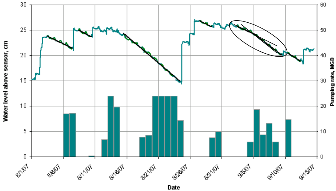
Figure 18 Impact of pumping on seepage rate. Calculated seepage rates for each period indicated in the figure are 0.21, 0.33, 0.66, 0.23, 0.30, 0.67, and 0.54 cm/d respectively. Higher rates coincide with extensive pumping. For example, in the circled region seepage rate doubles when the pump is turned on.
