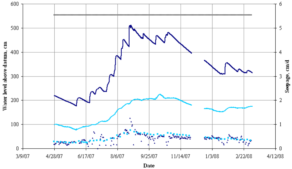
Figure 24 Well hydrographs for the sinkhole site. The straight line on top represents the land surface, the dark line is the surficial well hydrograph, the light line is the Floridan well hydrograph, the dark dots are seepage values calculated using the mass balance method, and the light dots are seepage values calculated using the head gradient method (Darcy's Law).
