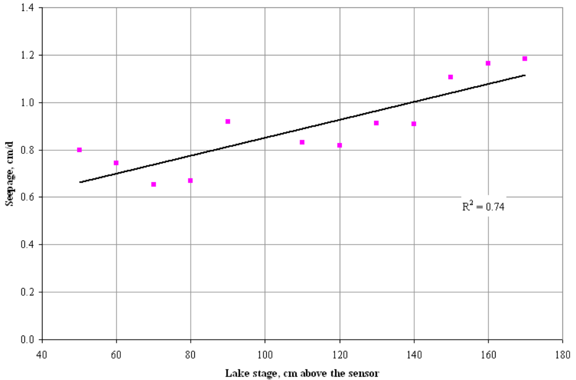
Figure 17 Botanical Gardens: seepage as a function of lake stage.
