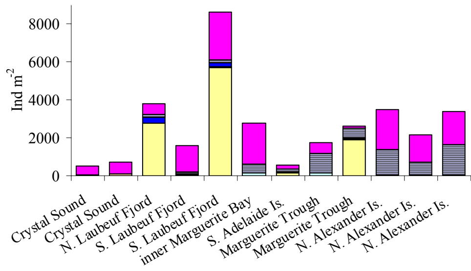
Figure 4.7a. Water column integrated abundances of zooplankton other than copepods and euphausiids ( \text{ind m}^{-2} ) from net hauls in the vicinity of Marguerite Bay during austral fall 2001 (top) and 2002 (bottom).
