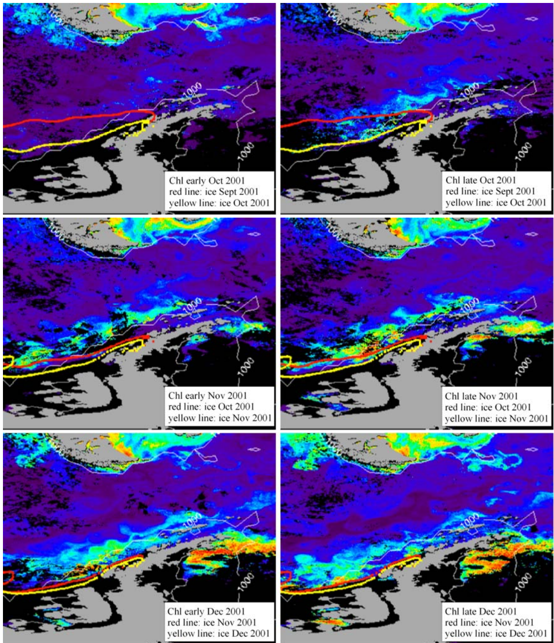
Figure 3.5b. Biweekly SeaWiFS chlorophyll concentrations (Chl, \text{mg m}^{-3} ) in October (Oct), November (Nov) and December (Dec) of 2001. The mean monthly location of the ice edge is also shown: the red line indicates the location of the ice edge during the preceding month, the yellow line represents the current month. The 1000 m isobath is indicated by the white line.
