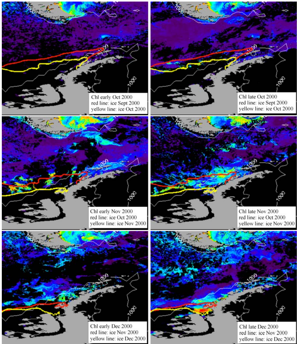
Figure 3.5a. Biweekly SeaWiFS chlorophyll concentrations (Chl, mg m -3 ) in October (Oct), November (Nov) and December (Dec) of 2000. The mean monthly location of the ice edge is also shown: the red line indicates the location of the ice edge during the preceding month, the yellow line represents the current month. The 1000 m isobath is indicated by the white line.
