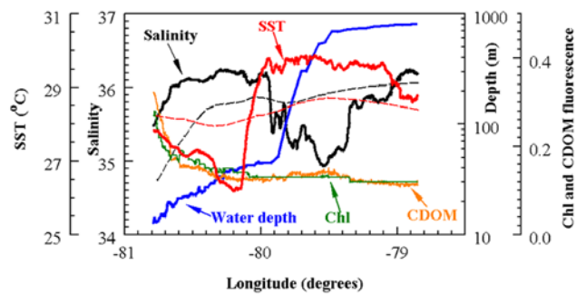
Figure 3. Near-surface water properties along the transect line in the SAB (11–12 August 2004, Figure 1b). Dashed lines indicate climatological means for temperature and salinity for this section of the Georgia shelf and Gulf Stream [Blanton et al. , 2003].
