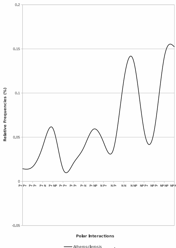
Figure 1. Relative Frequency distribution for lipoproteins related to atherosclerosis (Polanco et al. , 2015). The X-axis represents the 16 polar interactions.
