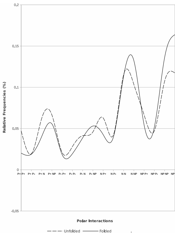
Figure 2. Relative frequency distribution for the unfolded and folded proteins (Polanco et al. , 2015a). The X-axis represents the 16 polar interactions.
