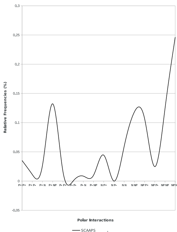
Figure 3. Relative frequency distribution for the selective cationic amphipathic antibacterial peptides (SCAAP) (Polanco & Samaniego, 2009). The X-axis represents the 16 polar interactions.
