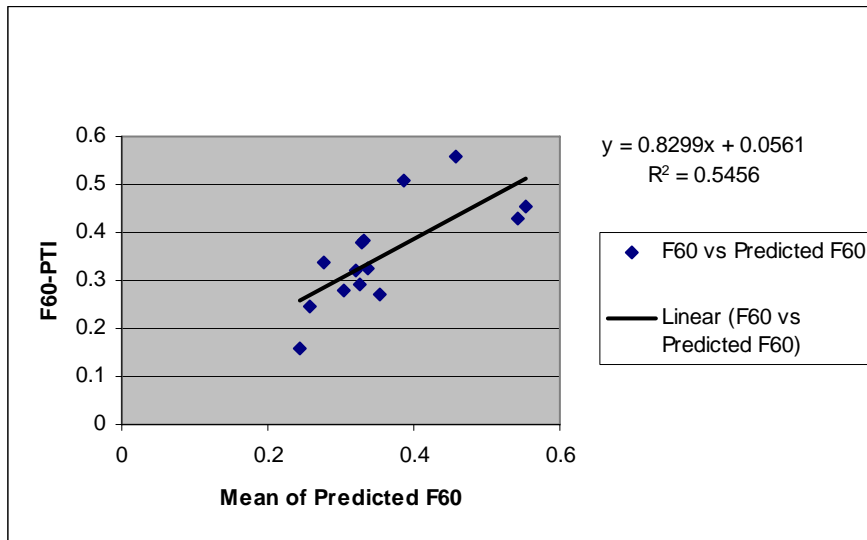
Figure 21 DFT F60 vs. Mean of Predicted F60 (NASA GT at 95 km/hr, DFT-PTI)
