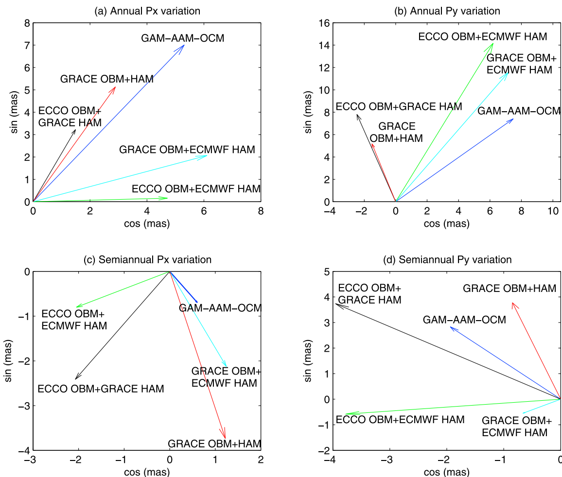
Figure 2. Phaser plots of (a) annual P_x , (b) annual P_y , (c) semiannual P_x , and (d) semiannual P_y excitation variations from geodetic observation residuals (GAM-AAM-OCM) (blue line), ECCO OBM plus ECMWF HAM (green line), ECCO OBM plus GRACE HAM (black line), GRACE OBM plus ECMWF HAM (cyan line), and GRACE OBM plus HAM (red line).
