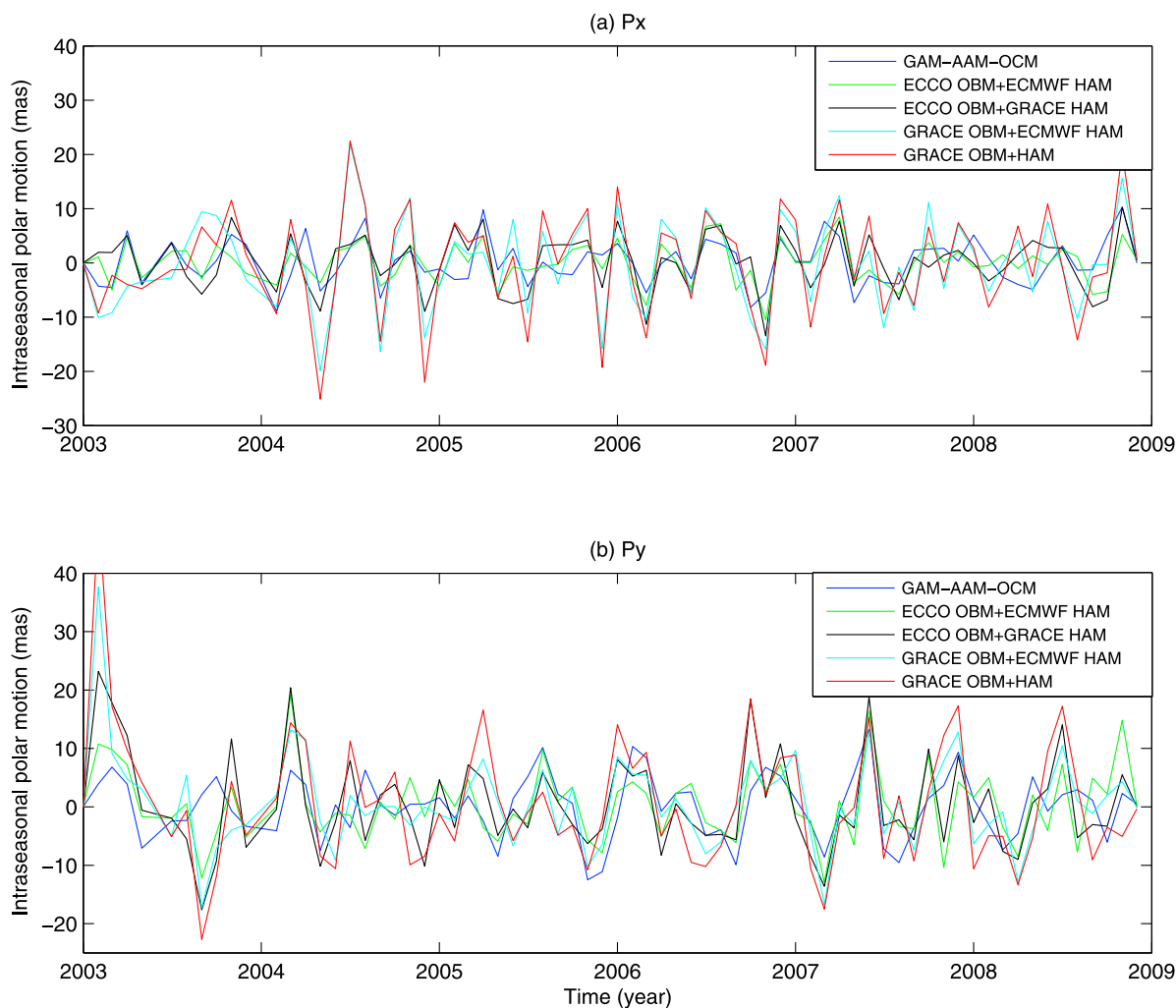
Figure 3. Intra-seasonal polar motion (a) P_x and (b) P_y from geodetic observation residuals (GAM-AAM-OCM) (blue line), ECCO OBM plus ECMWF HAM (green line), ECCO OBM plus GRACE HAM (black line), GRACE OBM plus ECMWF HAM (cyan line), and GRACE OBM plus HAM (red line). The mean, trend, annual, semiannual, and periods longer than 1 year have been removed from all time series by least squares fitting and a high-pass filter.
