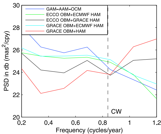
Figure 6. Power spectral density ( \text{mas}^2/\text{cpy} ) for polar motion P_x + iP_y of the geodetic observation residuals of GAM-AAM-OCM (blue line) with GRACE and models' estimates. A mean, trend, and seasonal signals at the annual and semiannual frequencies have been removed from all time series prior to the fast Fourier transform analysis. The vertical dashed line is at the Chandler wobble period.
