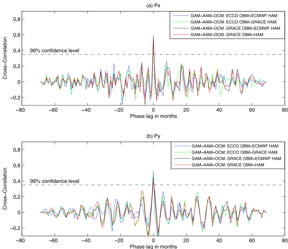
Figure 4. Cross-correlation coefficients for the intraseasonal polar motion (a) P_x and (b) P_y between geodetic observation residuals of GAM-AAM-OCM and ECCO OBM plus ECMWF HAM (blue line), ECCO OBM plus GRACE HAM (green line), GRACE OBM plus ECMWF HAM (black line), GRACE OBM plus HAM (red line), respectively. The two dashed lines in Figures 4a and 4b represent the 99% confidence levels.
