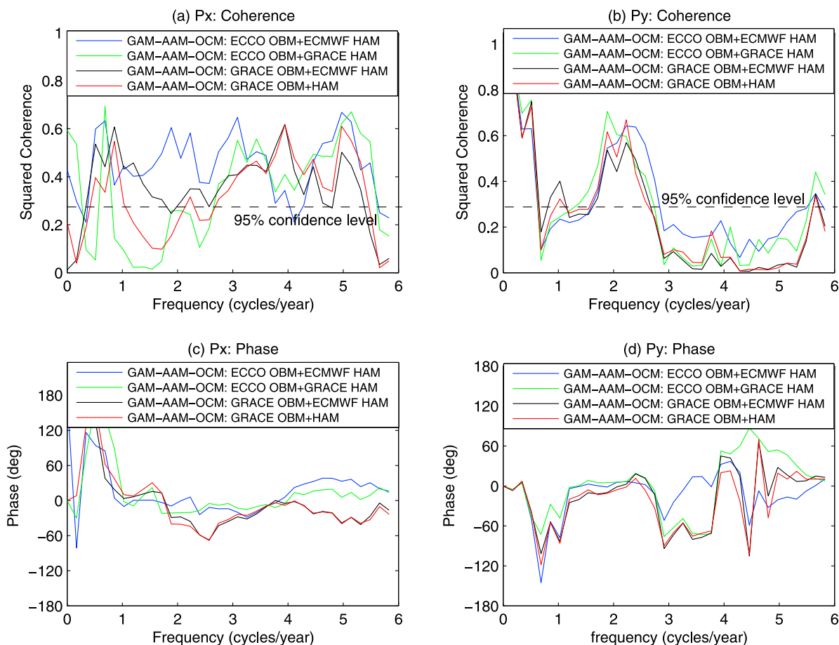
Figure 5. Magnitude and phase of the squared coherence of GAM-AAM-OCM with GRACE and model excitations. Annual, semiannual, and periods longer than 1 year have been removed from all time series by least squares fitting and high-pass filter. A mean and trend are also removed. The dashed lines in Figures 5a and 5b represent the 95% confidence levels.
