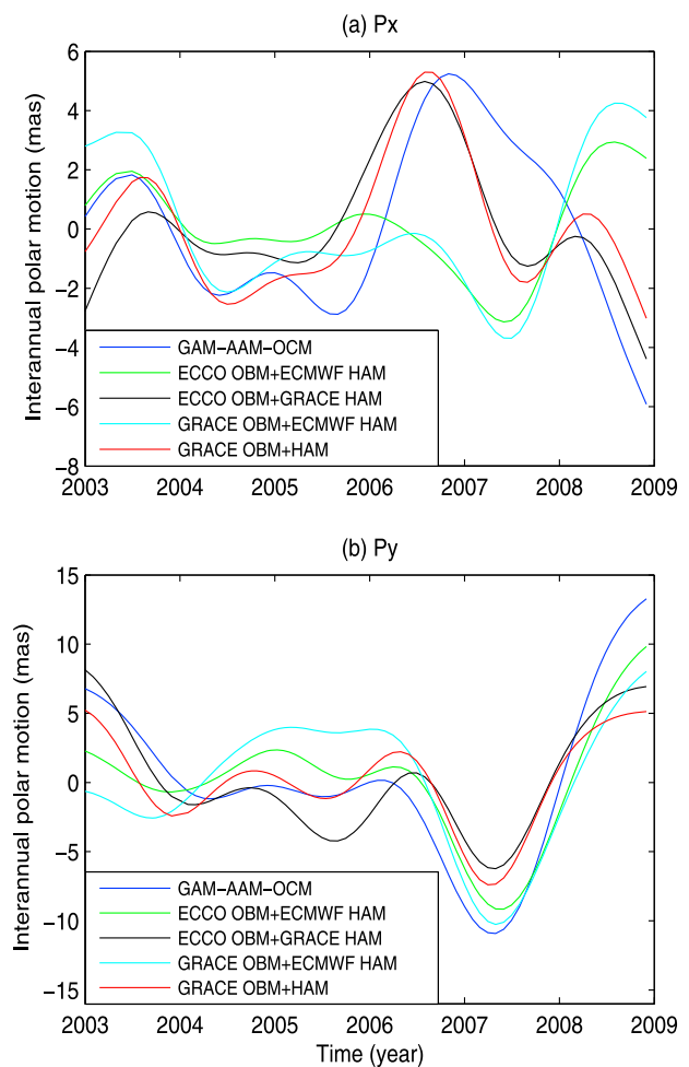
Figure 7. Residual interannual excitations in (a) P_x and (b) P_y after removing seasonal variations and smoothing over 1 year.
