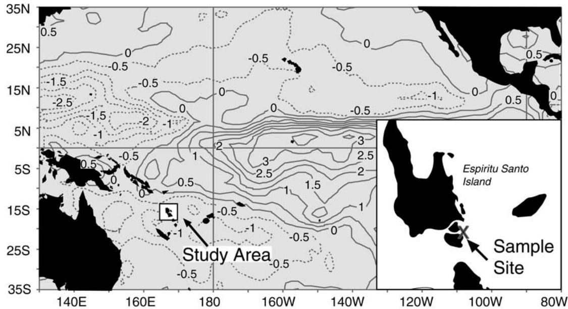
Figure 1. Sample site map superimposed on a contour map of March–November average precipitation rate anomaly (mm/day) during ENSO warm phase years shows that Vanuatu is well situated to experience precipitation anomalies during El Niño events. Data from the NCEP/NCAR reanalysis model [Kalnay et al. , 1996] were provided by the NOAA-CIRES Climate Diagnostics Center, Boulder, Colorado, from their Web site at http://www.cdc.noaa.gov/ . ENSO years considered are 1958, 1966, 1969, 1973, 1983, 1992, and 1998, compared against the 1968–1996 average.
