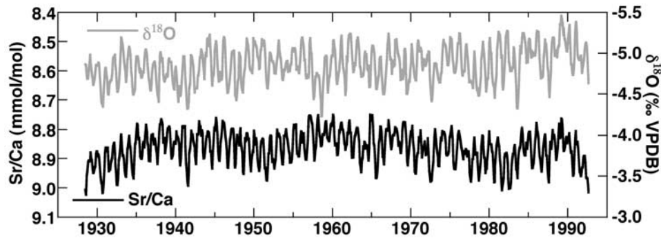
Figure 2. Sr/Ca and \delta^{18}\text{O} variations in a Porites lutea from Malo Channel, Vanuatu. Clear annual cycles in the geochemistry and cross-referencing the geochemistry with the annual density bands ensures a robust age model.
