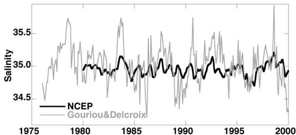
Figure 3. A comparison of monthly hindcast model salinity (NCEP; Behringer et al. [1998]) and monthly gridded ship of opportunity data [Gouriou and Delcroix, 2002]. Note the large difference in variability between the two SSS data sets from the same region of the surface ocean. Such differences have the capability to introduce nontrivial confusion in climate proxy interpretations.
