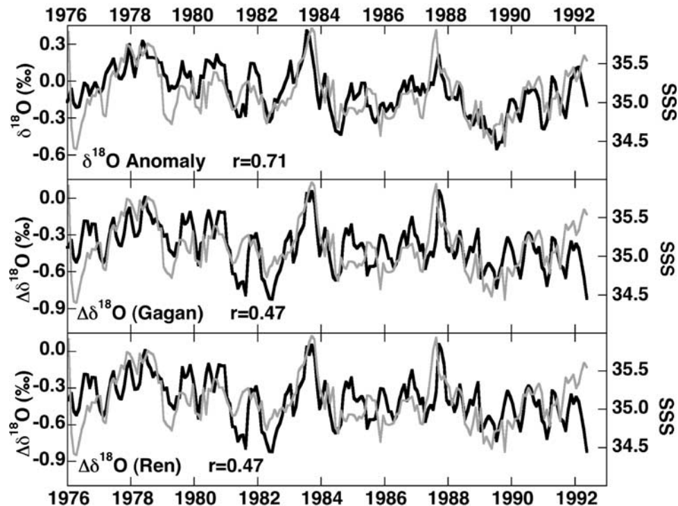
Figure 4. Comparison of three coral-based reconstructions of seawater \delta^{18}\text{O} (heavy black lines) and instrumental SSS (thin gray line; Gouriou and Delcroix [2002]). The top panel is the \delta^{18}\text{O} anomaly (monthly averages 1928–1992 subtracted out), the middle panel uses the method proposed by McCulloch et al. [1994] and expanded by Gagan et al. [1998], and the bottom panel uses the method of Ren et al. [2002]. The correlation coefficients ( r ) for each proxy of salinity are calculated after detrending the data and normalizing by the standard deviations of each time series.
