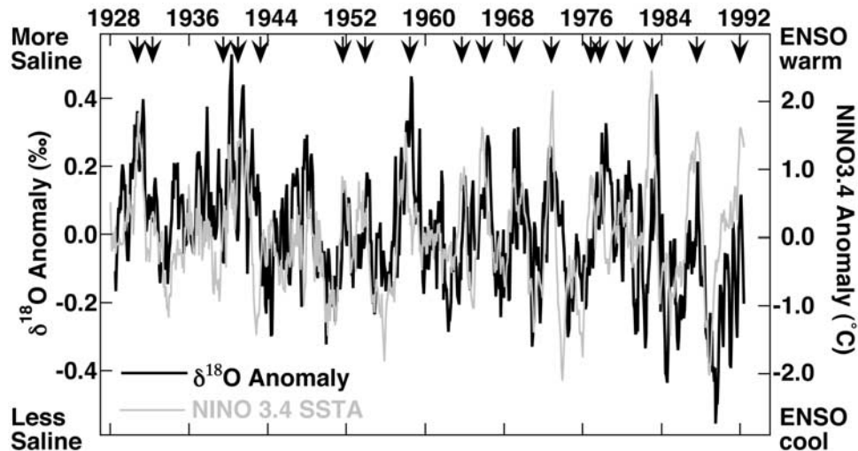
Figure 5. Santo coral \delta^{18}\text{O} anomaly plotted versus Niño 3.4 region SSTA. The \delta^{18}\text{O} curve has been shifted forward in time by 6 months to compensate for a 6 month lag time between the salinity response at Vanuatu to changes in temperature in the Niño 3.4 region. ENSO warm phase events (El Niño) in the eastern Pacific are correlated with increased salinity in the western Pacific and are noted by arrows along the top of the graph.
