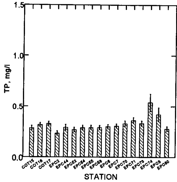
Figure 31. Comparison of mean values and standard errors for TP concentrations measured at the COT compliance monitoring stations and all EPC stations in Hillsborough Bay for the year 1997.
