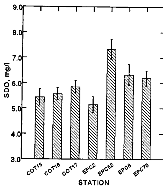
Figure 35. Comparison of mean values and standard errors for SDO concentrations measured at the COT compliance monitoring stations and the group of EPC stations close to the Howard F. Curren WWTP discharge site for the year 1997.
