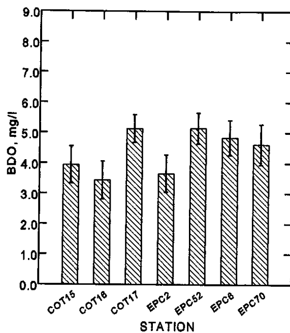
Figure 37. Comparison of mean values and standard errors for BDO concentrations measured at the COT compliance monitoring stations and the group of EPC stations close to the Howard F. Curren WWTP discharge site for the year 1997.
