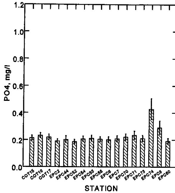
Figure 33. Comparison of mean values and standard errors for PO4 concentrations measured at the COT compliance monitoring stations and all EPC stations in Hillsborough Bay for the year 1997.
