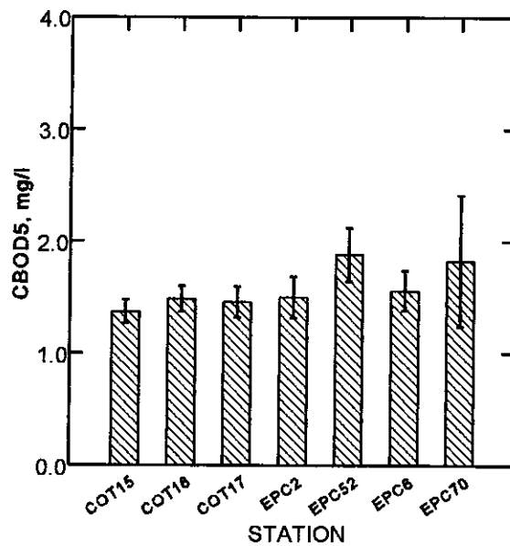
Figure 34. Comparison of mean values and standard errors for CBOD5 concentrations measured at the COT compliance monitoring stations and the group of EPC stations close to the Howard F. Curren WWTP discharge site for the year 1997.
