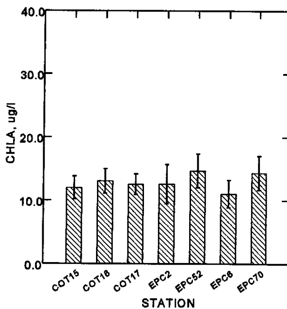
Figure 38. Comparison of mean values and standard errors for CHLA concentrations measured at the COT compliance monitoring stations and the group of EPC stations close to the Howard F. Curren WWTP discharge site for the year 1997.
