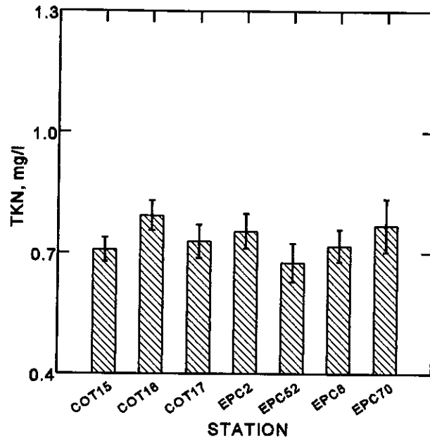
Figure 29. Comparison of mean values and standard errors for TKN concentrations measured at the COT compliance monitoring stations and the group of EPC stations close to the Howard F. Curren WWTP discharge site for the year 1997.
