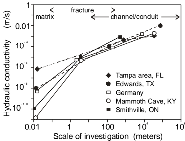
Figure 11 Scaling in hydraulic conductivity in the Edwards Aquifer and in other karst aquifers (after Worthington et al., 2002).
