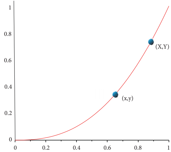
FIGURE 1: Abel's problem.
