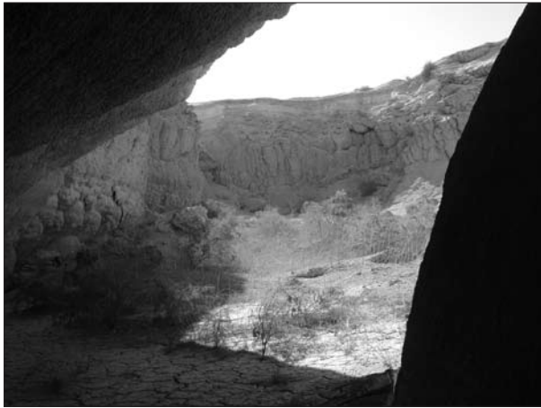
Fig. 6: View of the northern section of Sinkhole 2 from underneath the solid tufa showing the vertical tufa walls.
