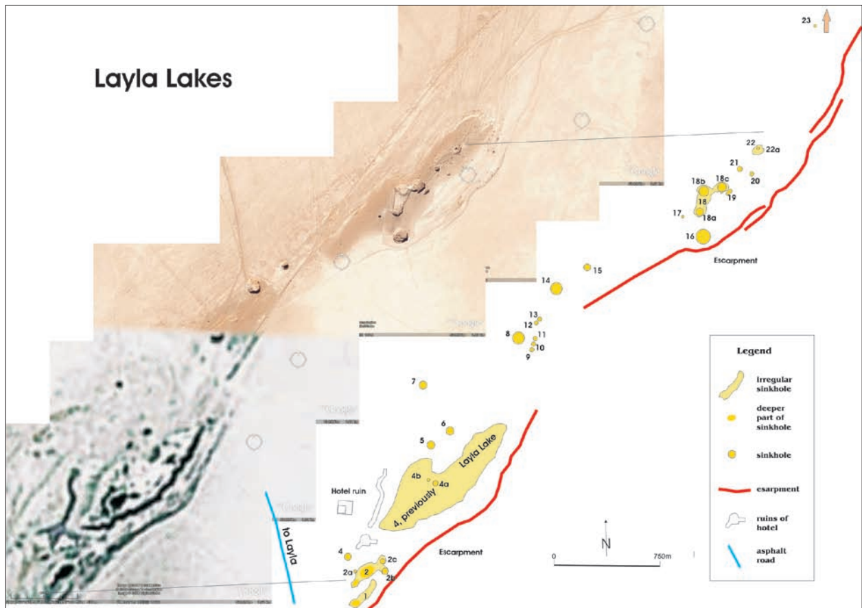
Fig. 4: Google Earth view of the Layla Lakes area and annotated map of sinkholes.
