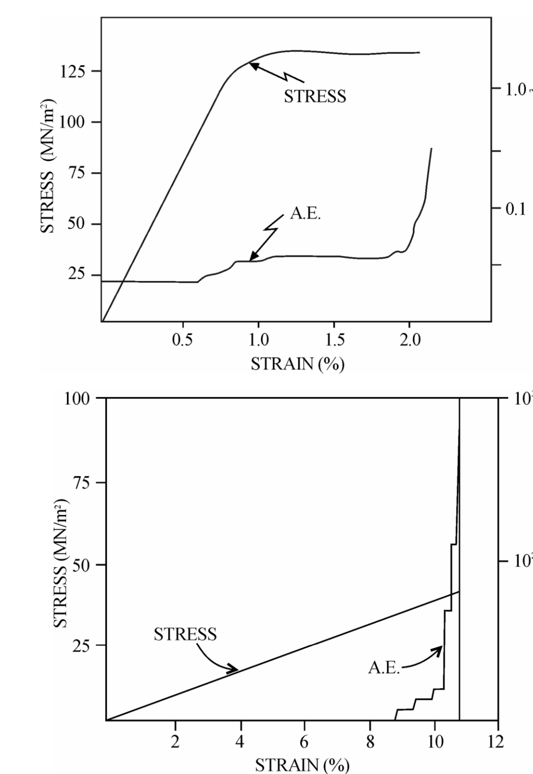
Figure 3. Graph of control specimen (top) and decalcified specimen (bottom) depicting stress v. strain and AE counts v. strain. Shrivastava, S., & Prakash, R. (2009). Adapted from JBSE
