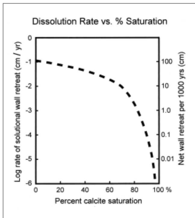
Fig. 1: Rates of limestone dissolution vs. percent calcite saturation at 10° C and 0.01 atm CO 2 partial pressure (calculated from references in text).
