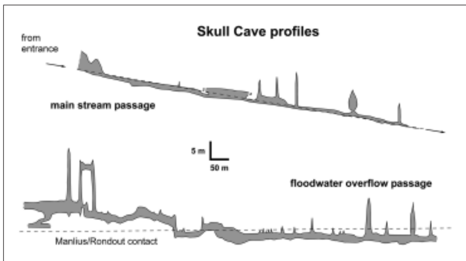
Fig. 12: Profiles of the main stream passage and the main east-west passage of Skull Cave, showing floodwater fissures in ceiling.
