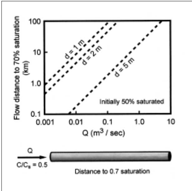
Fig. 4: Distance of penetration of highly aggressive flow into water-filled conduits. In this example, incoming allogenic water is assumed to be already 50% saturated (concentration / saturation concentration = 0.5). The graphs show the distance required for the water to reach only 70% saturation, beyond which the dissolution rate begins to decrease rapidly. Variations with discharge ( Q ) and passage diameter ( d ) are shown. A typical cave stream can penetrate a great distance while retaining most of its initial aggressiveness.
