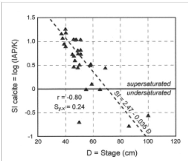
Fig. 14: Calcite saturation index (SI calcite) of allogenic water entering Mystery Cave vs. river stage on West Fork of Root River. Equilibria calculated by Palmer and Palmer (1993) from chemical data by Grow (1986). Approximate conversion from C/C_s in Fig. 4 is SI = \log [(C/C_s)^{2.86}] .
