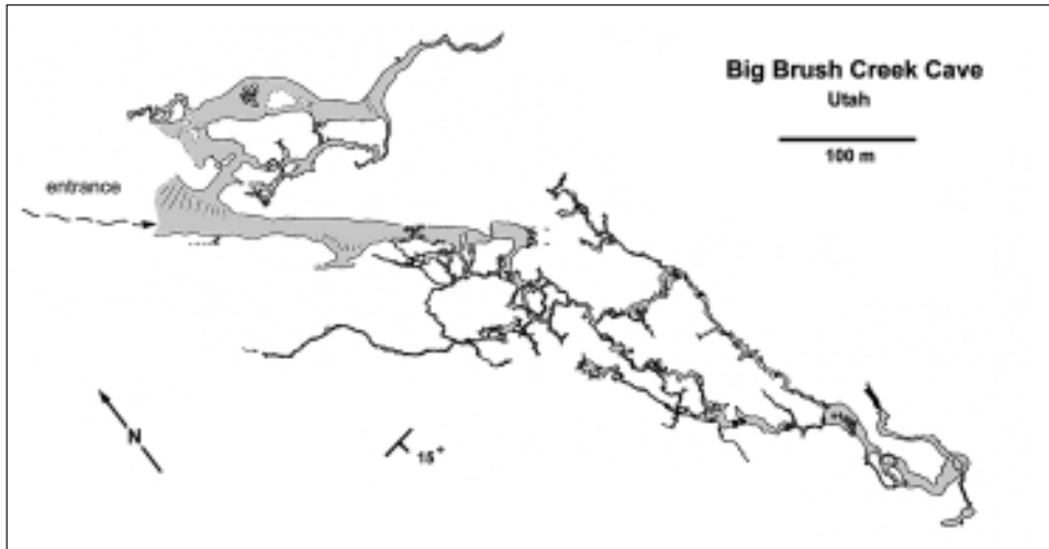
Fig. 15: Partial map of Big Brush Creek Cave, Utah (from Palmer, 1975).
