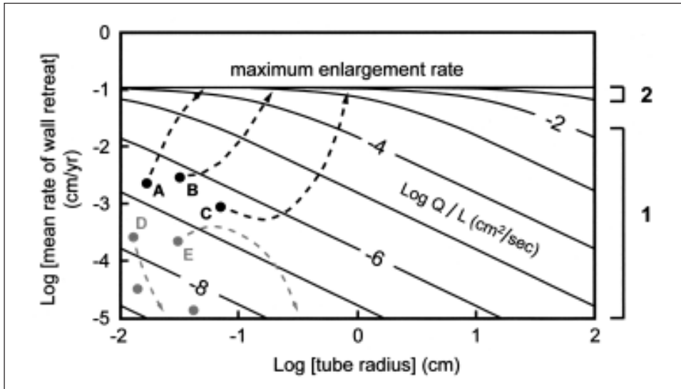
Fig. 2: Mean rates of solutional wall retreat in limestone conduits (from Palmer, 1991). Q/L = ratio of discharge to flow distance. Early stages of karst aquifer development are represented by zone 1, which includes a great variety of dissolution rates. Q increases with time in only a few conduits, allowing them to grow at a faster rate (A, B, C), while others stagnate at low and usually diminishing enlargement rates. Only those that reach the maximum rate (zone 2) grow into traversable caves. Graphs are similar for conduits with non-circular cross sections, but the lines have gentler slopes.
