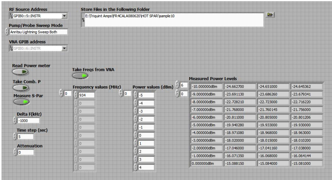
Figure A.2 – Application that Automates the HOT S-Parameters Measurement
