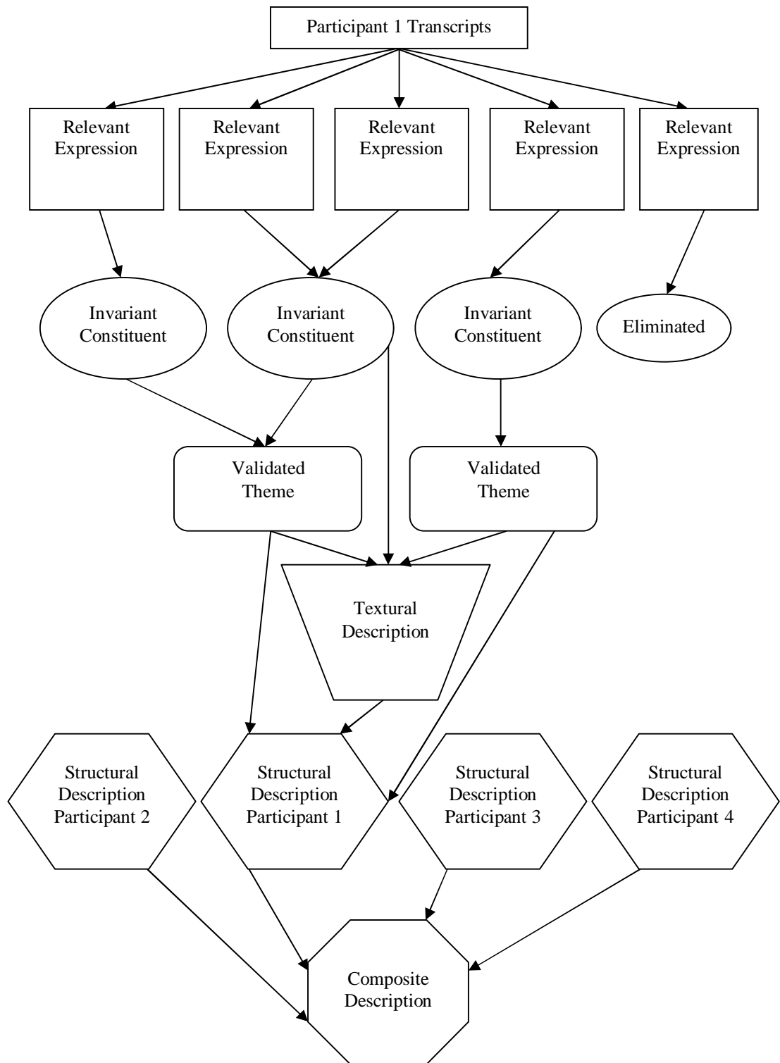
Figure 2: Application of the van Kaam (1959, 1966) Method of Phenomenological Analysis
