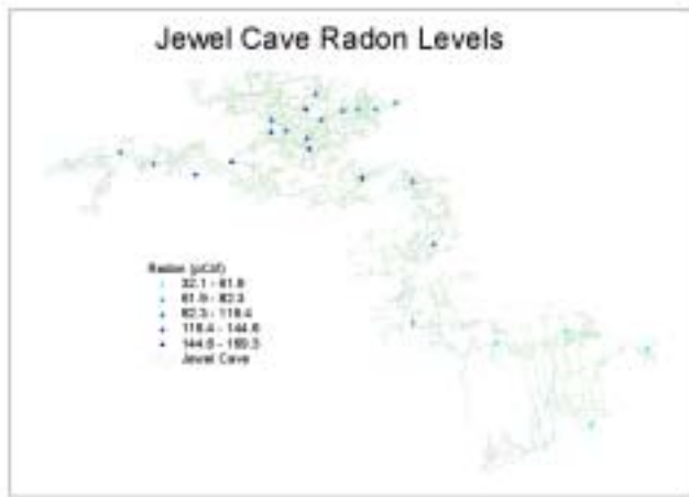
Figure 2: Radon levels in Jewel Cave.
