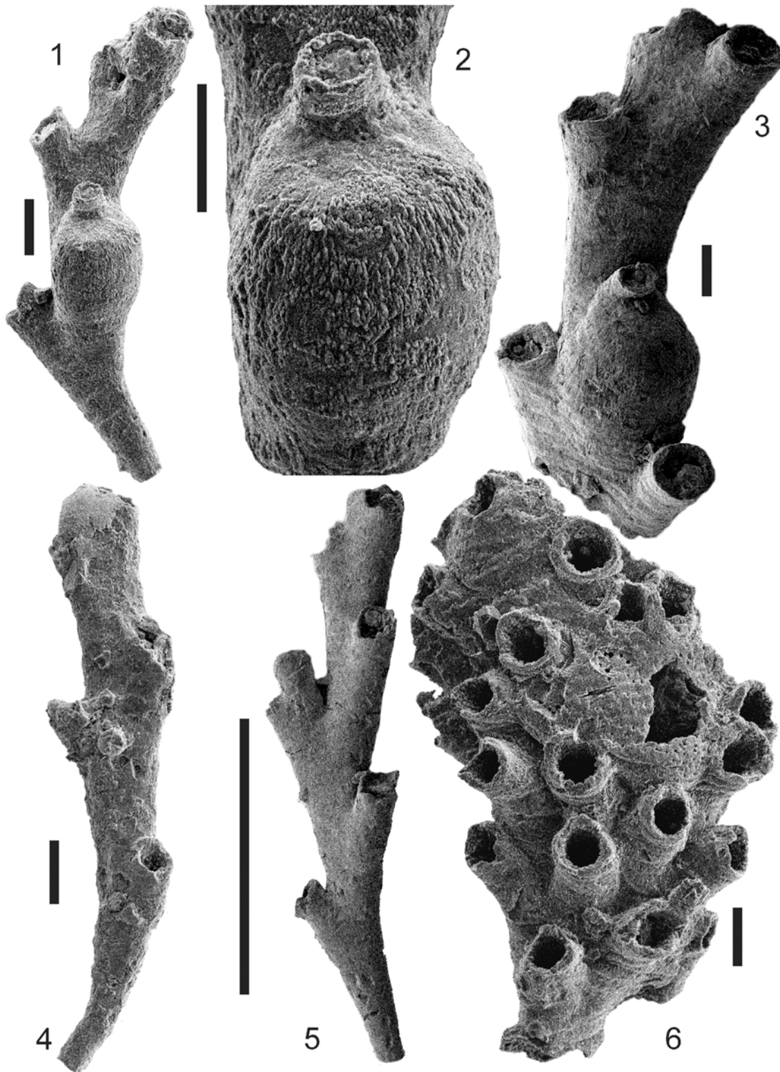
Plate I. Crisia romanica sp. nov. from the Răcăștia 2, sample 7
