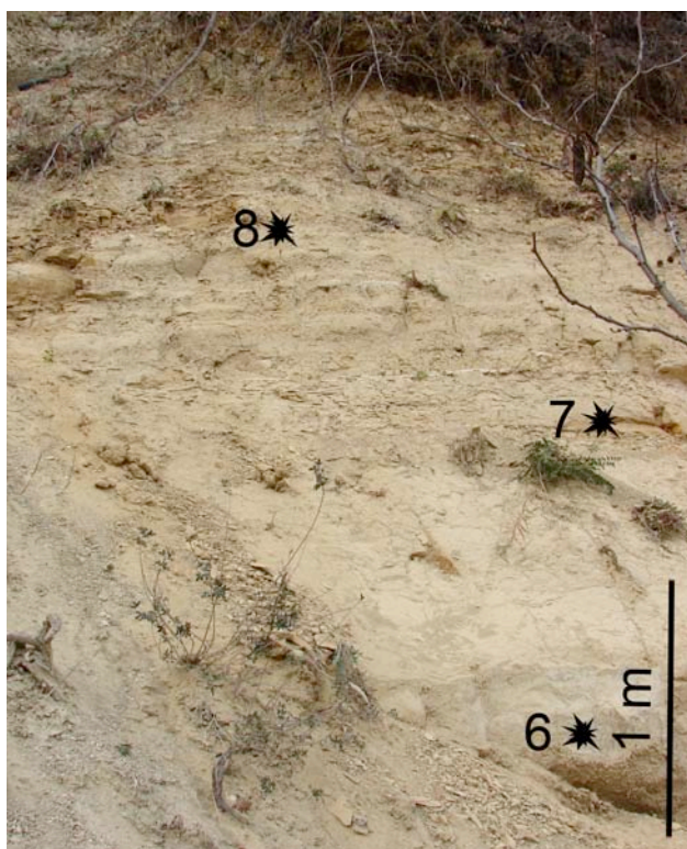
Fig. 3. Photograph of section Răcăștia 2, showing the main lithological features and the position of the samples 6 to 8.
