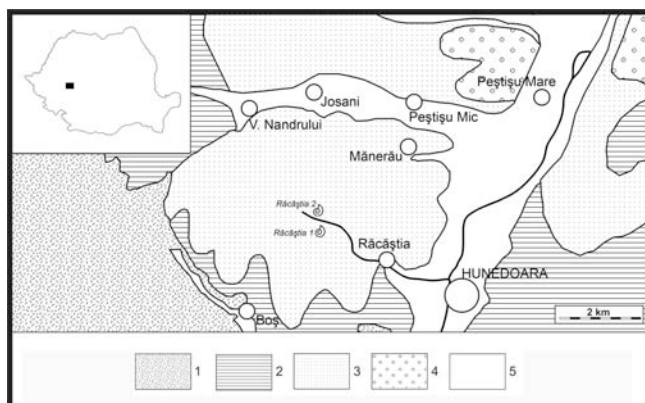
Fig. 1. Simplified geological map showing the location of sampled outcrops: 1. metamorphic rocks, 2. Badenian, 3. Sarmatian, 4. Pleistocene, 5. Holocene (based on Gherasi et al., 1968).
