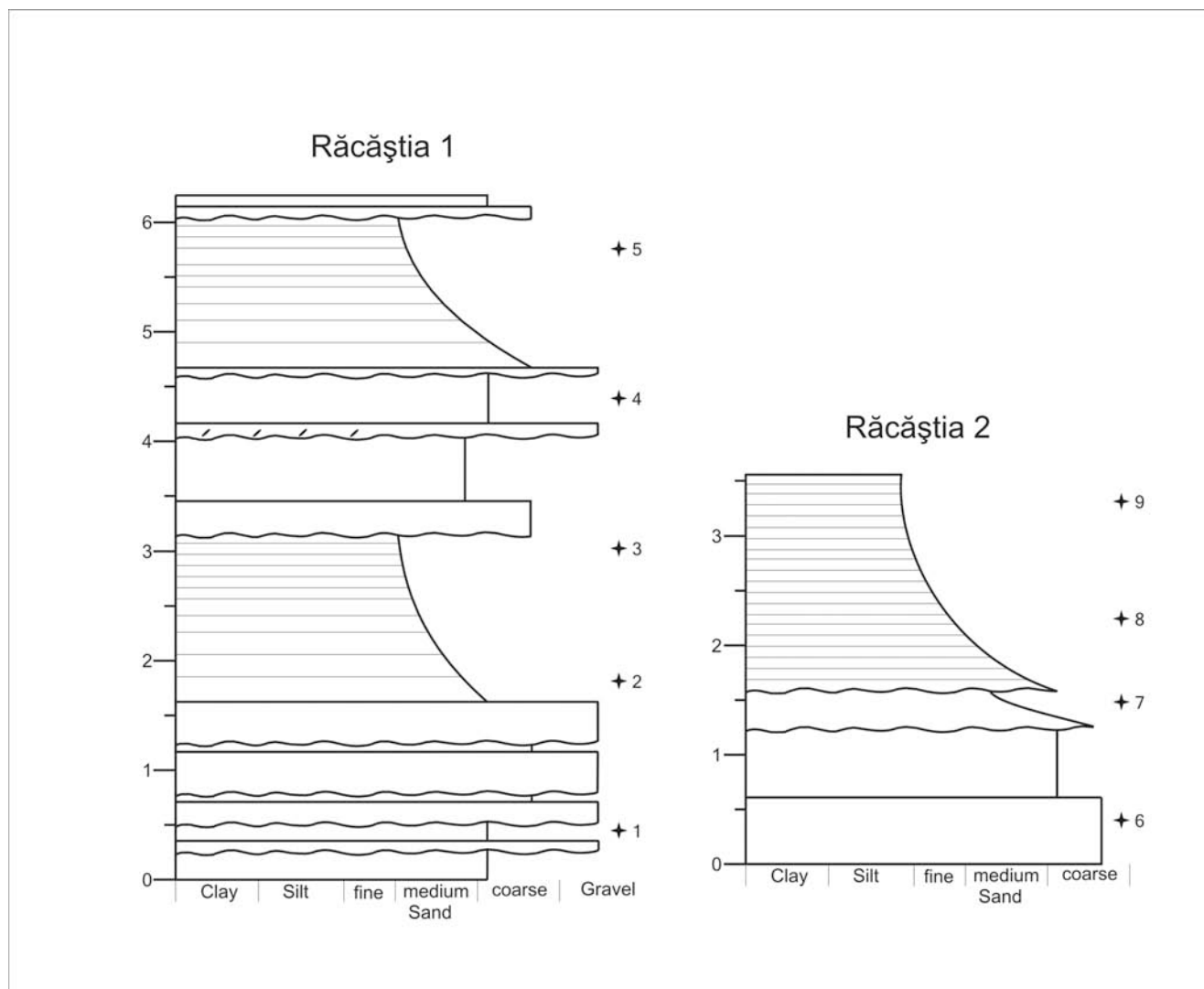
Fig. 2. Lithological section of the studied localities. Position of samples indicated by asterisks and numbers (for detailed explanations concerning lithology see the text).
