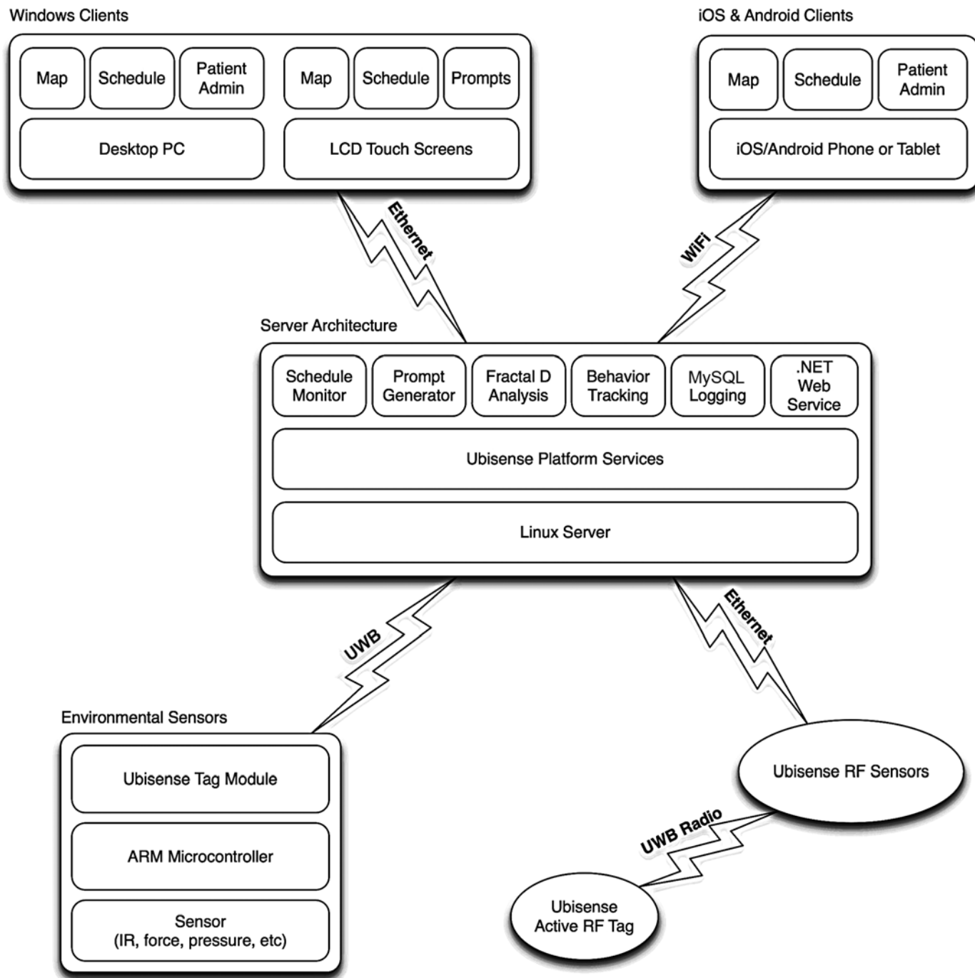
Figure 1. Smart home architecture. Combination of environmental and location sensors connected to Linux server running Ubisense core platform services (Ubisense Ltd; Cambridge, England) as well as custom smart home applications for behavior monitoring, prompting, and data analysis. End user applications run on Windows (Microsoft; Redmond, Washington), iOS (Apple, Inc; Cupertino, California), and Android (Google, Inc; Menlo Park, California) devices. Admin = administration, Fractal D = fractal dimension, IR = infrared, LCD = liquid crystal display, PC = personal computer, RF = radio frequency, UWB = Ubisense wireless backchannel.
